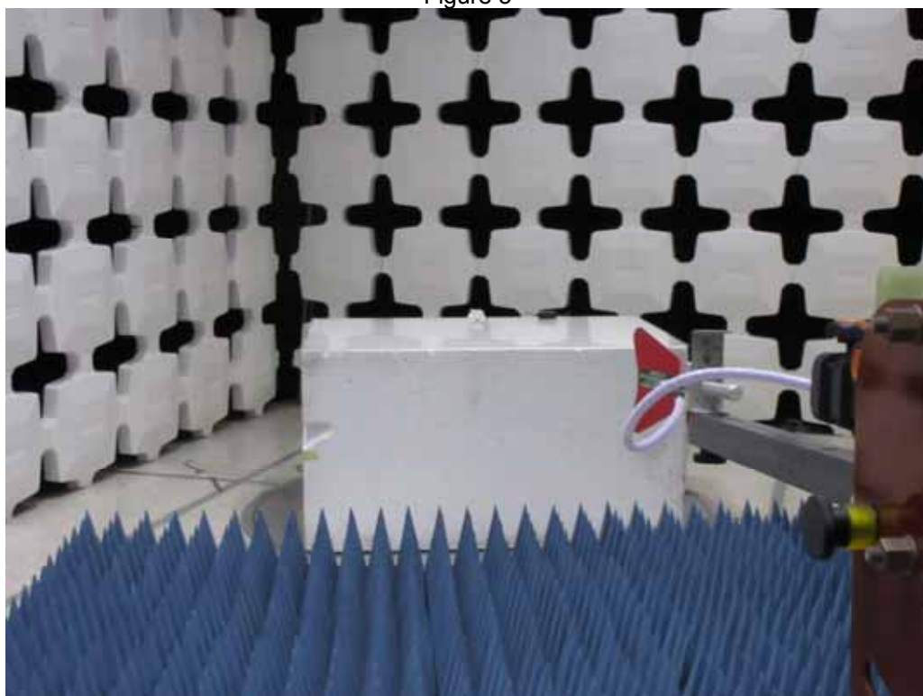
Test Setup for Receiver Radiated Emissions – 1GHz to 2GHz, Horizontal Polarization
