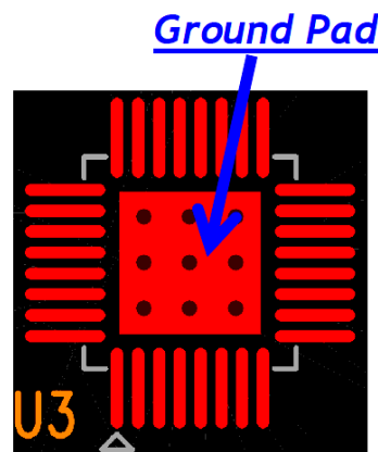
Figure 5-6. ALC5623 PCB footprint
