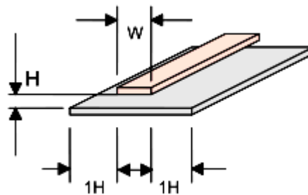
Figure 4-1. Microstrip Structure
