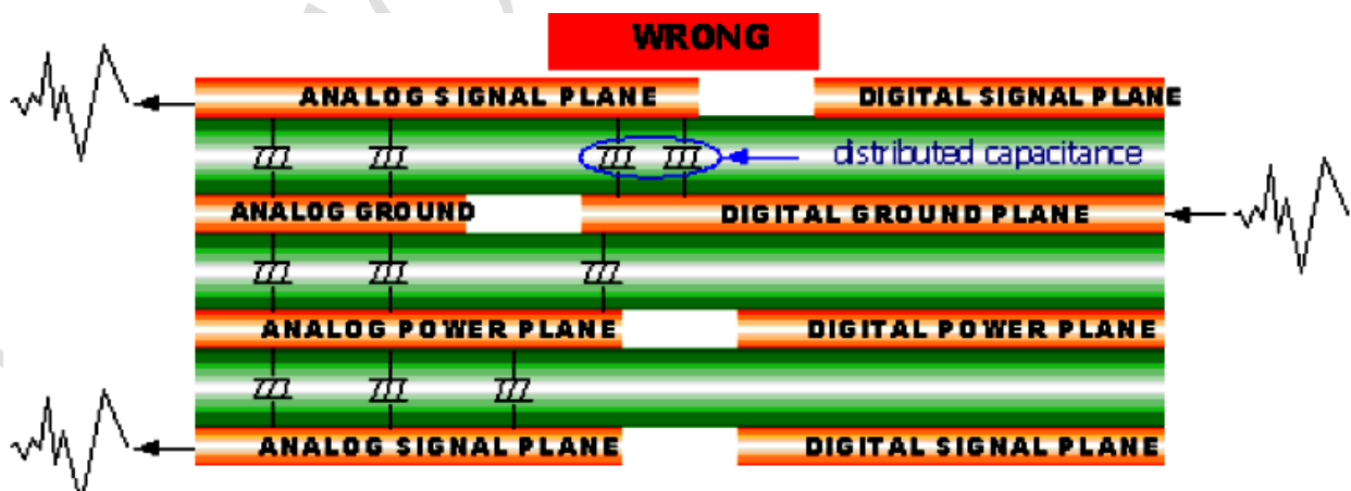
Figure. 5-3 Side view of PCB, the “ Wrong ” separation of analog and digital plane.
