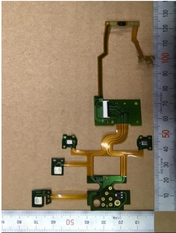
FPC_TOP_C_B
