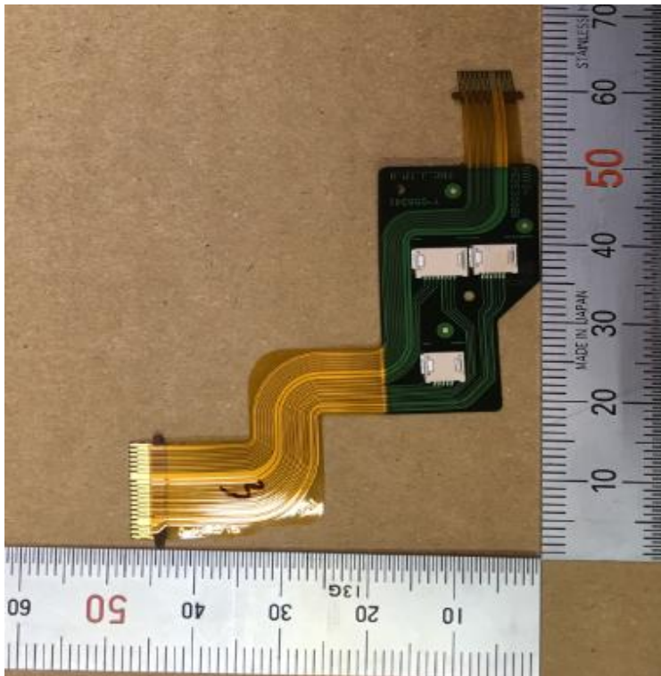
FPC_TOP_R_A
