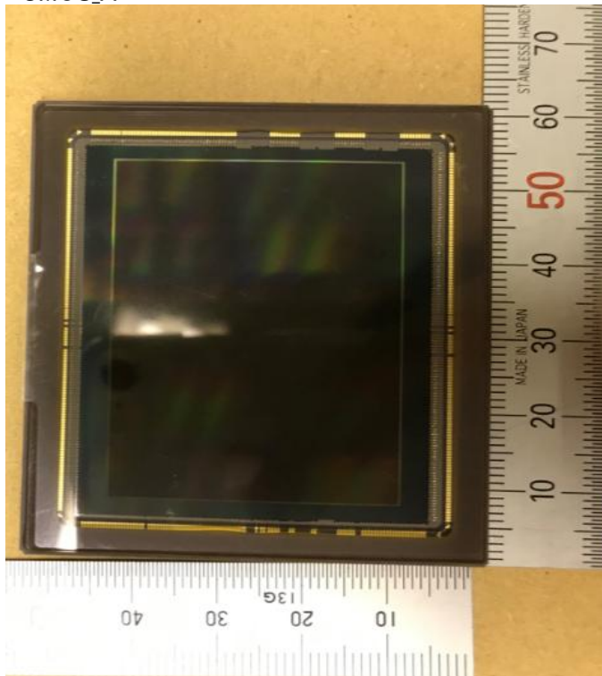
CMOS_B
