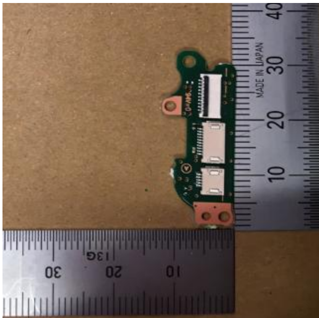
TOP_BTN_PWB_B
