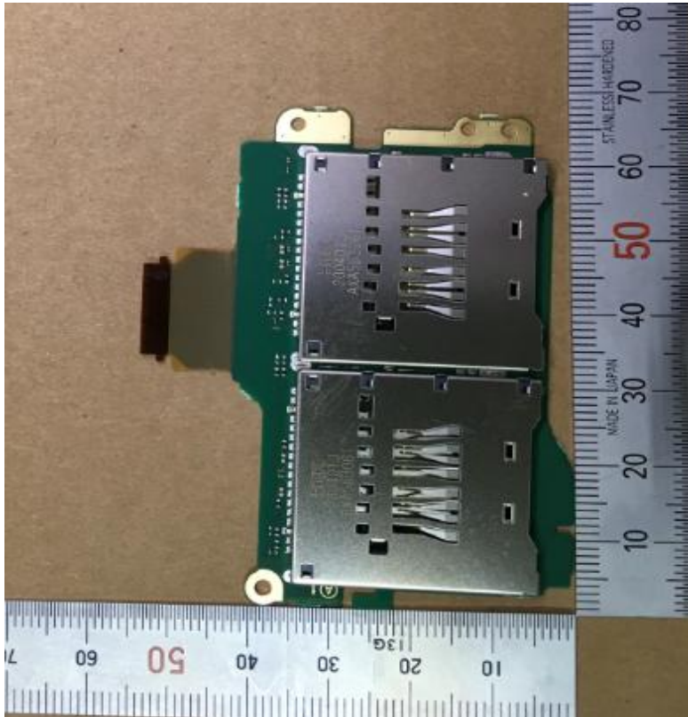
PWB_SD_A
