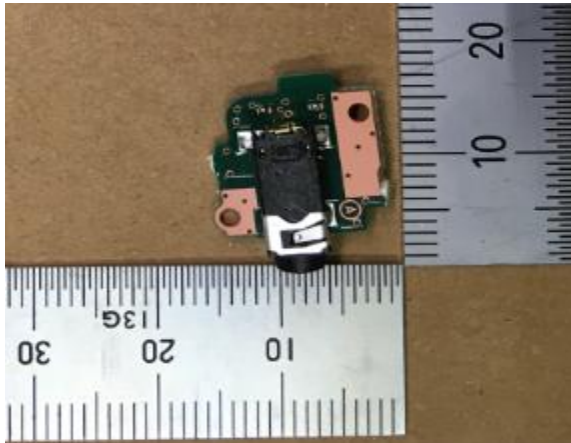
RR_JACK_A
