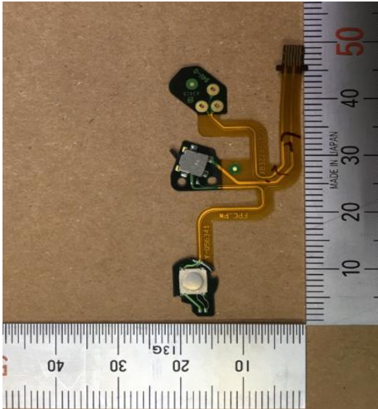
FPC_PW_A
