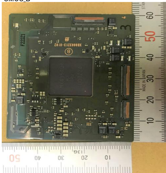
CMOS_B
