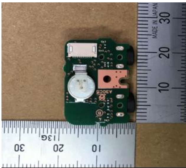
MIC_PWB_B
