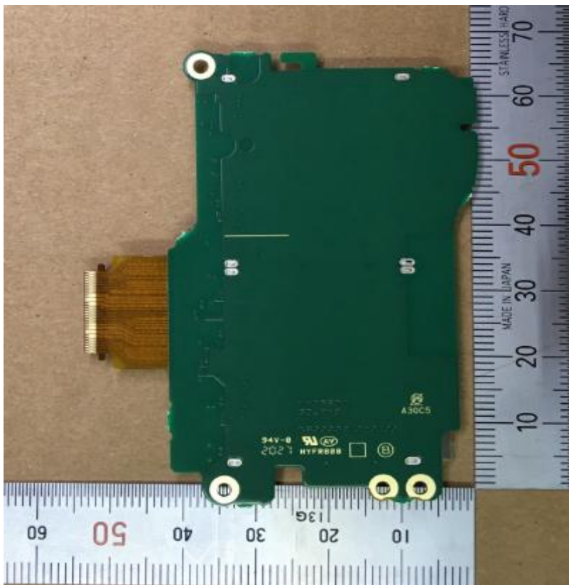
PWB_SD_B
