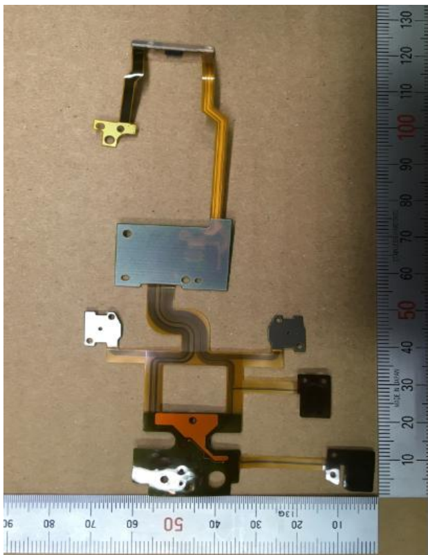
FPC_TOP_C_B
