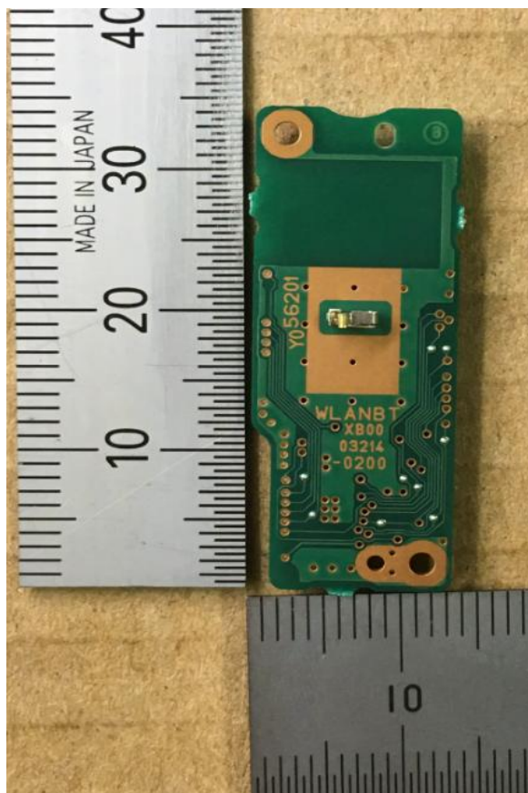
PWB_WLAN_B
