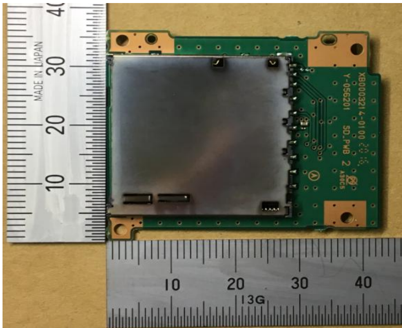
PWB_SD_A
