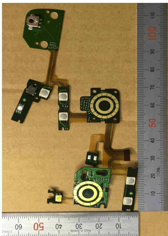
FPC_TOP_R_A
