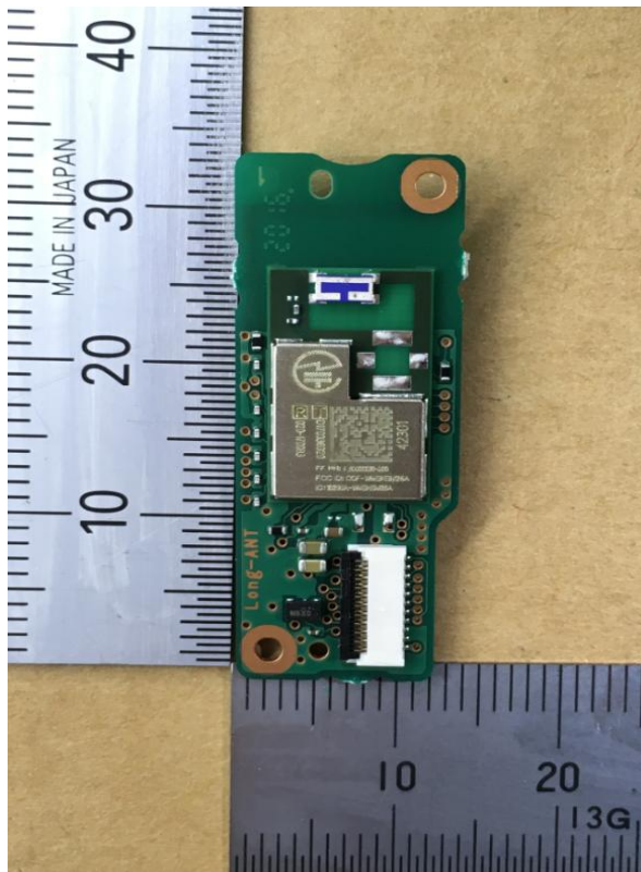
PWB_WLAN_A
