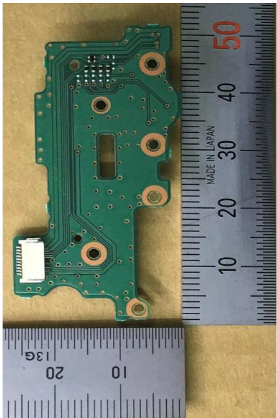
PWB_REAR_B
