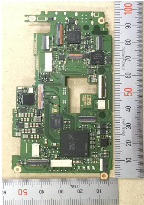
PWB MAIN_A
