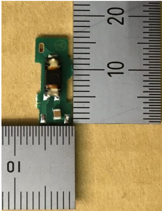
PWB_TRIGGER_A
