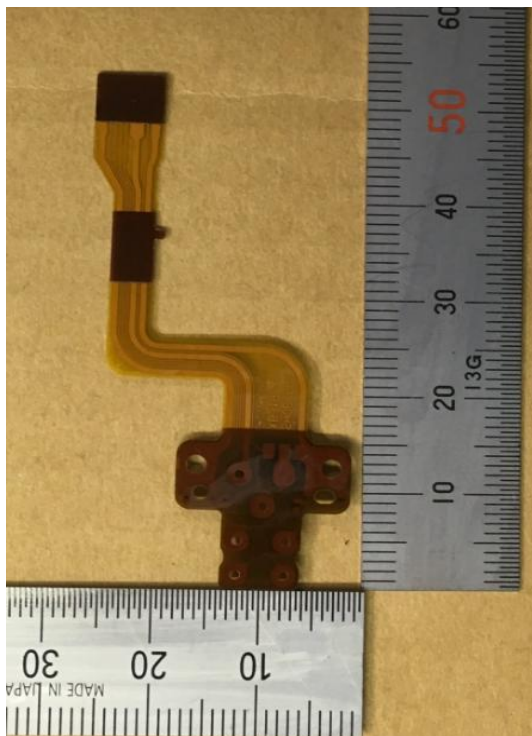
SHOE_FPC_B
