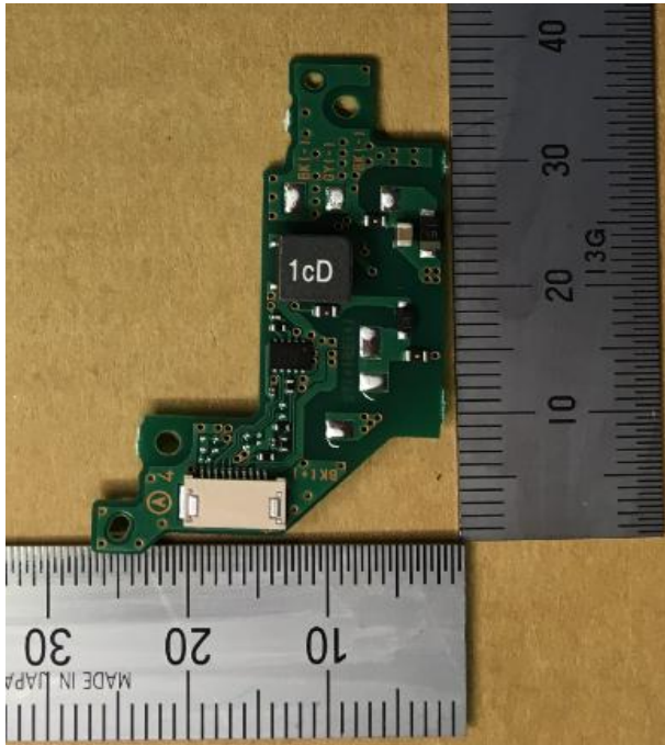
PWB_FLASH_A
