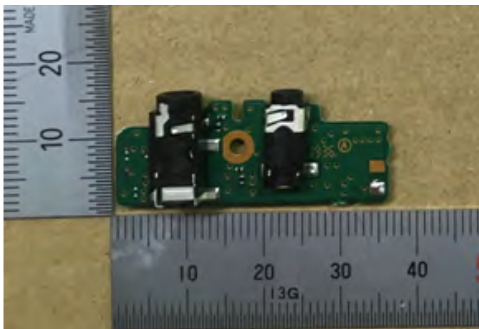
PWB MIC_A
