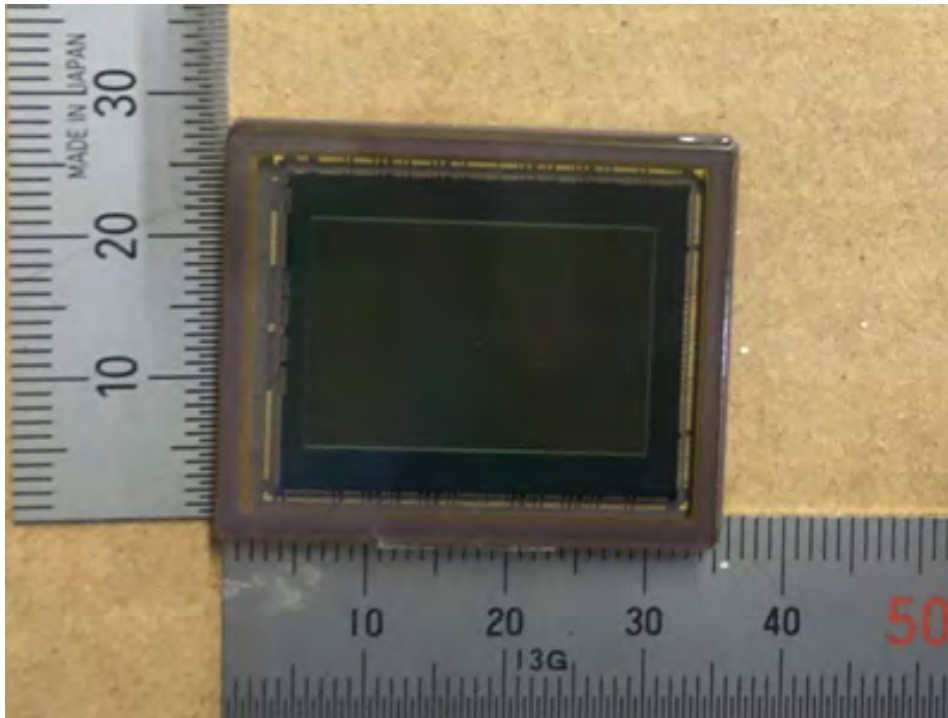
PWB CMOS_A
