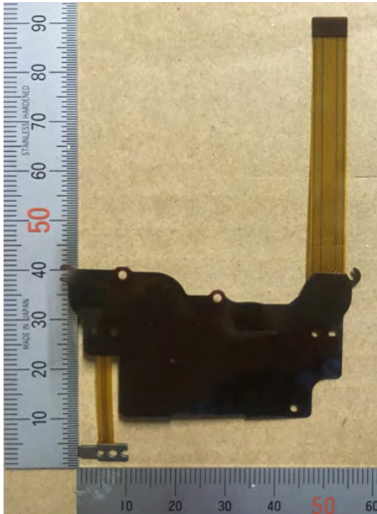
FPC REAR_B
