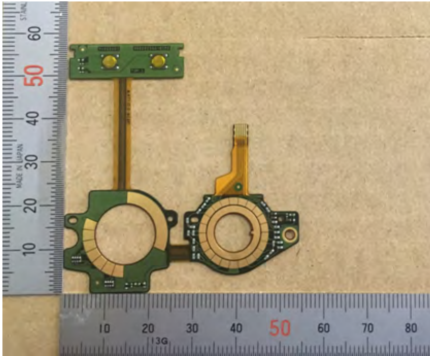
FPC TOP L_A
