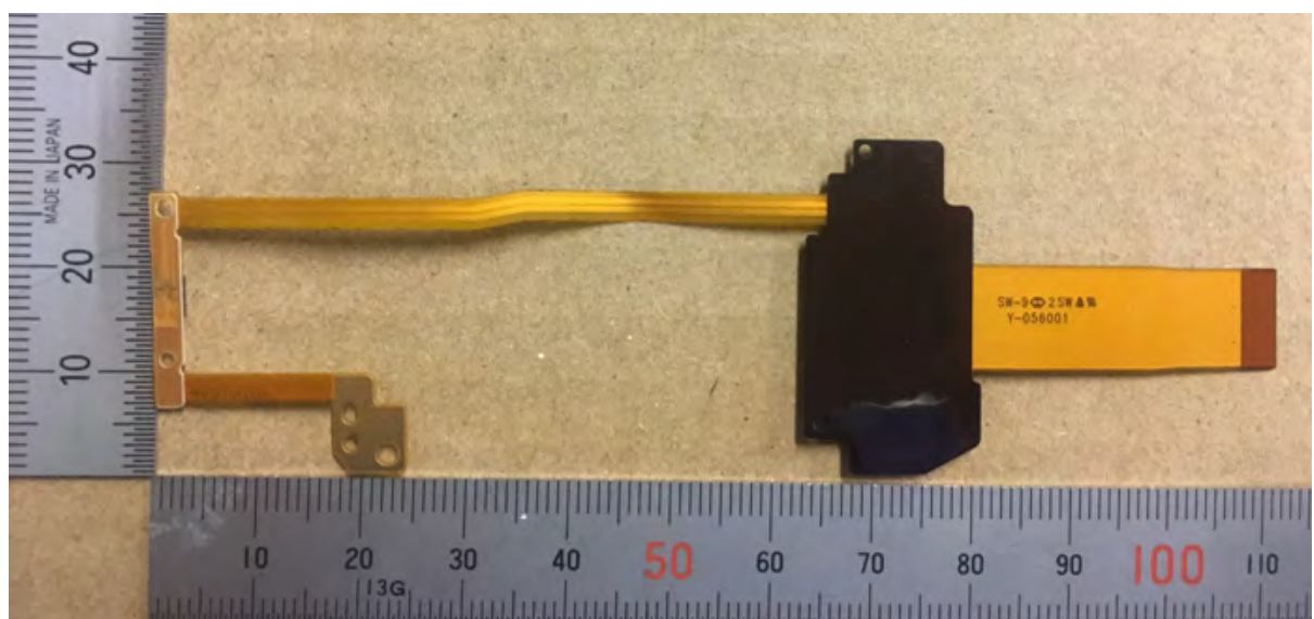
FPC JOINT EVF_B
