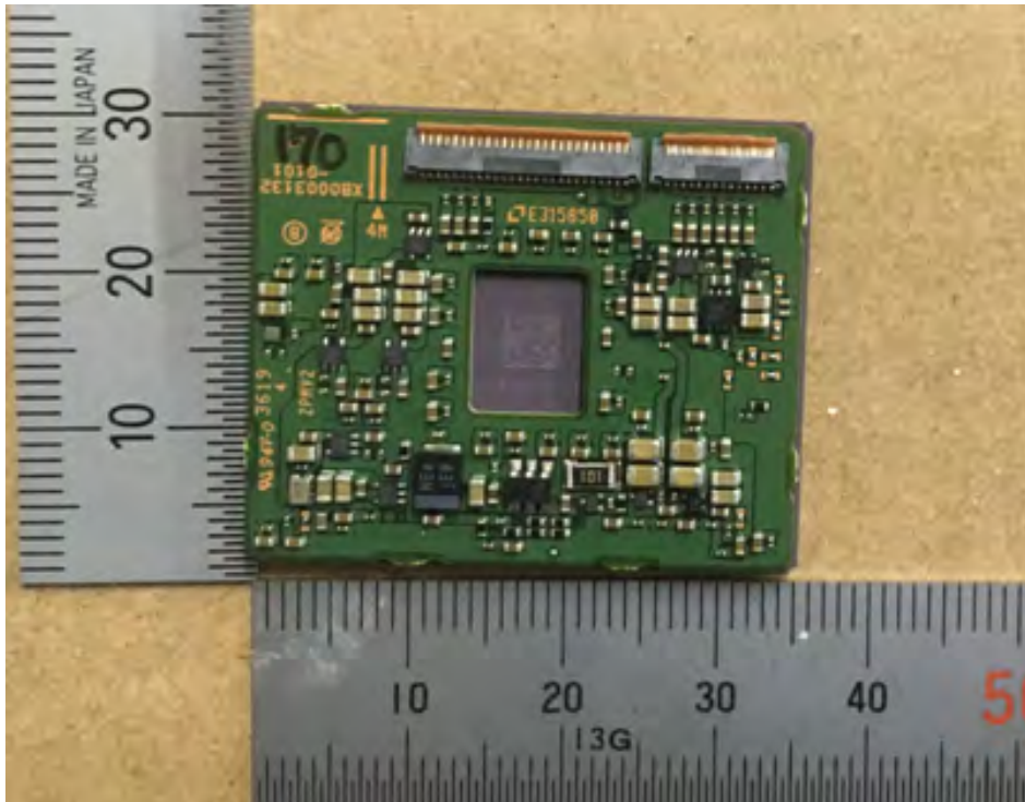
PWB CMOS_B
