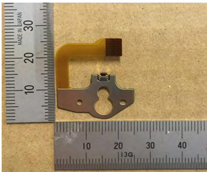
FPC COMMAND_F_B
