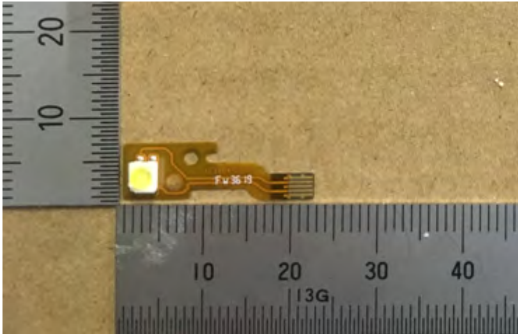
FPC LED_A
