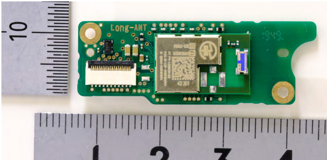
PWB WLAN_A
