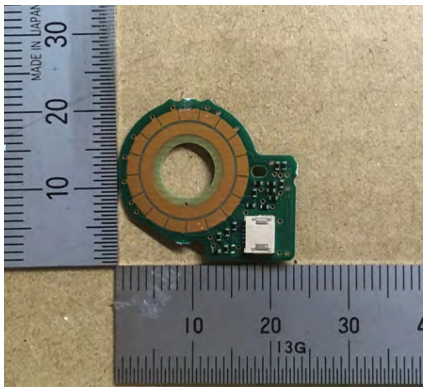
PWB DIAL SS_A
