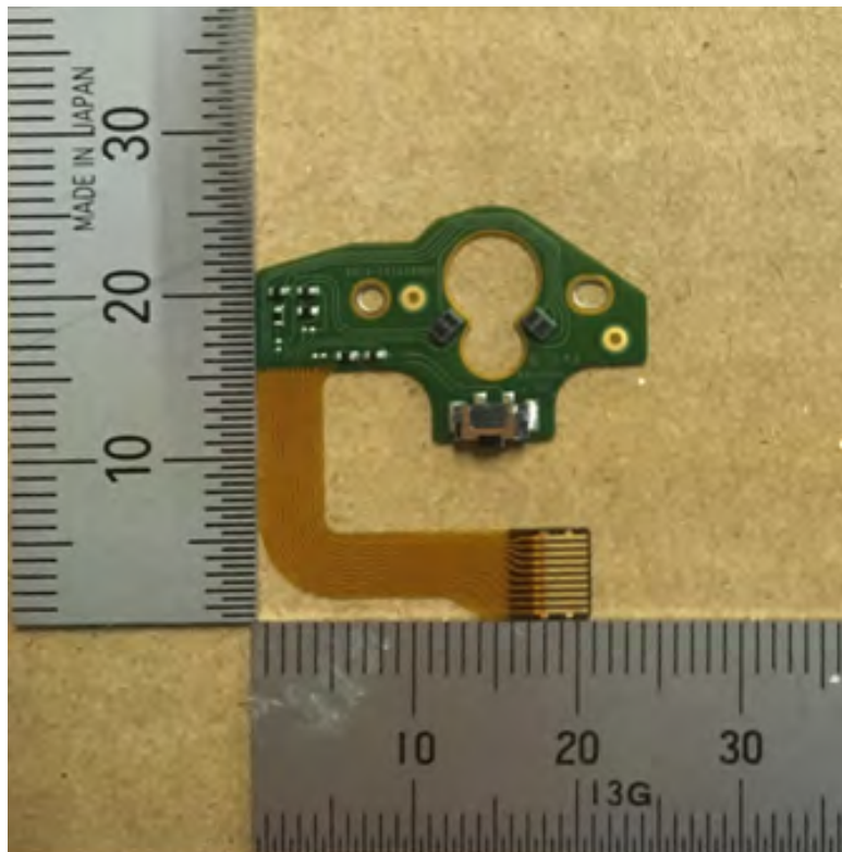
FPC COMMAND_F_A
