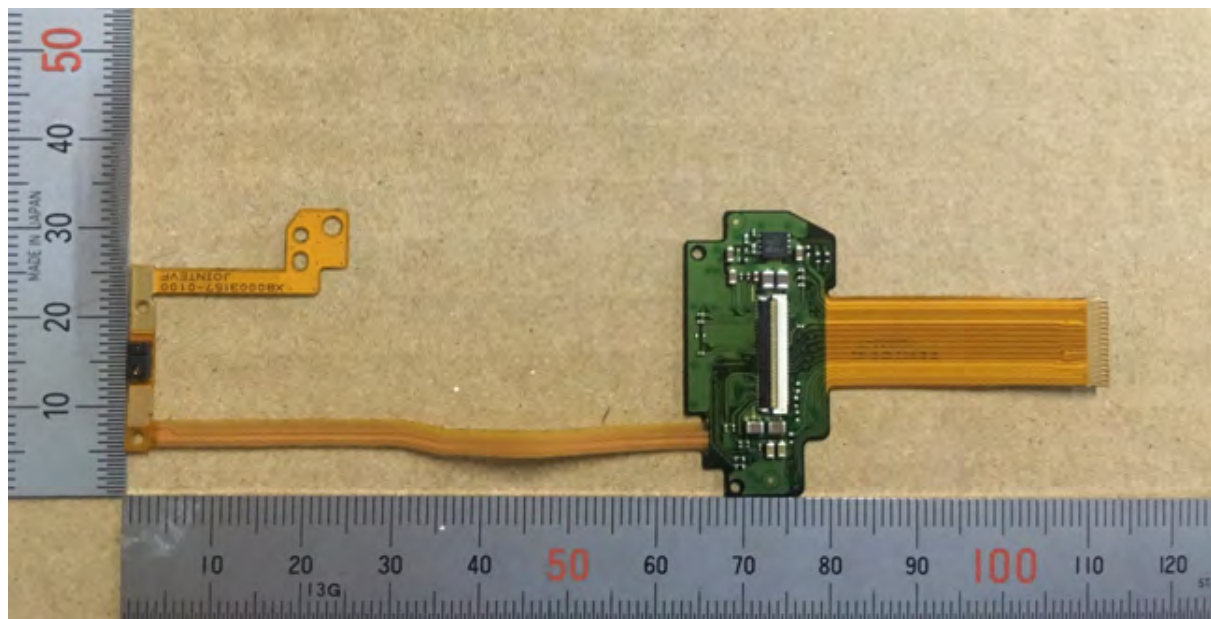
FPC JOINT EVF_A
