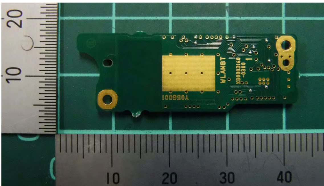
PWB WLAN_B
