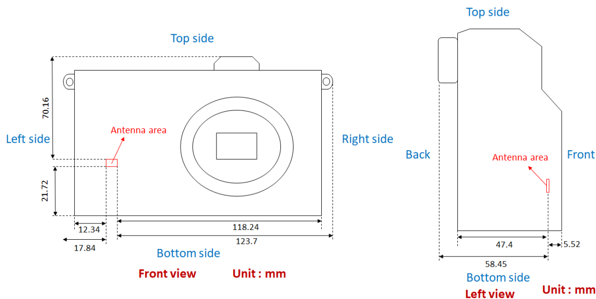
Fig.9 Antenna position
