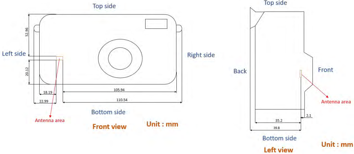
Fig.9 Antenna position
