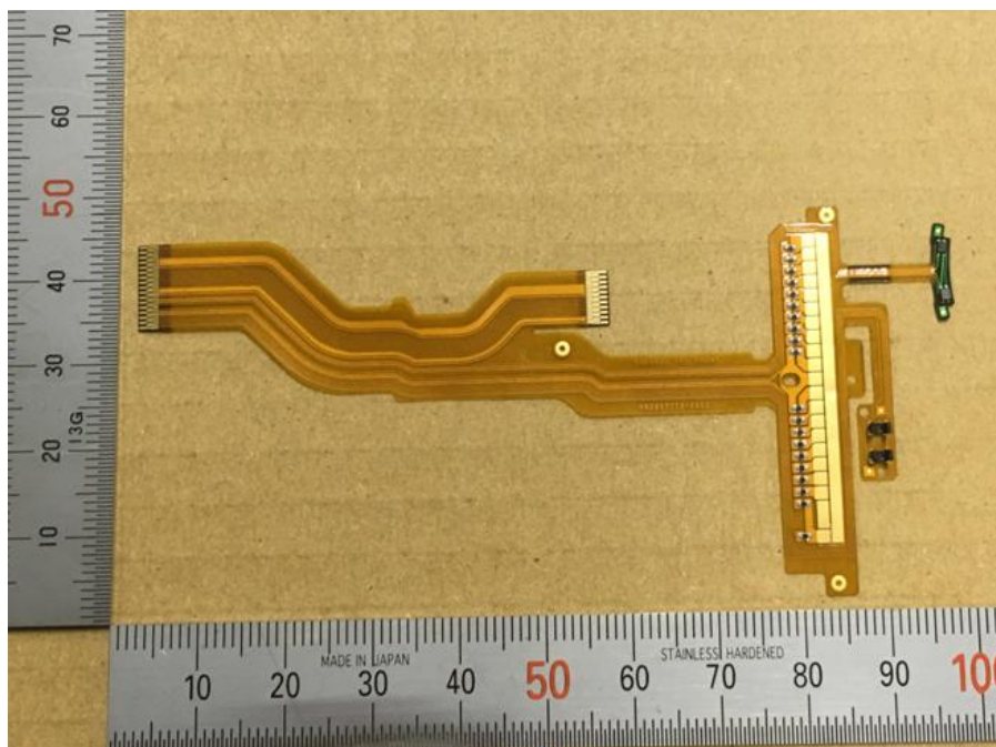
FPC_FRONT_A
