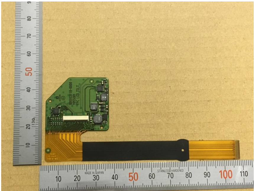
FPC_TILT_LCD_B
