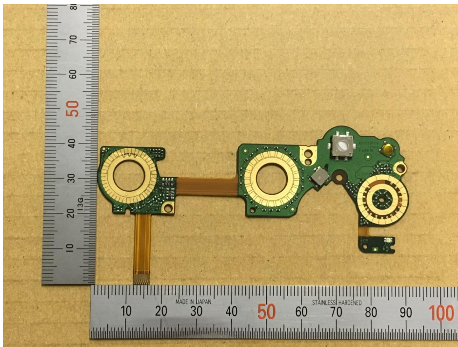
FPC_TOP_B
