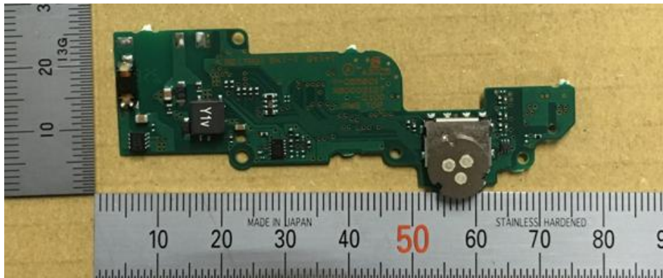
PWBTOP_A
