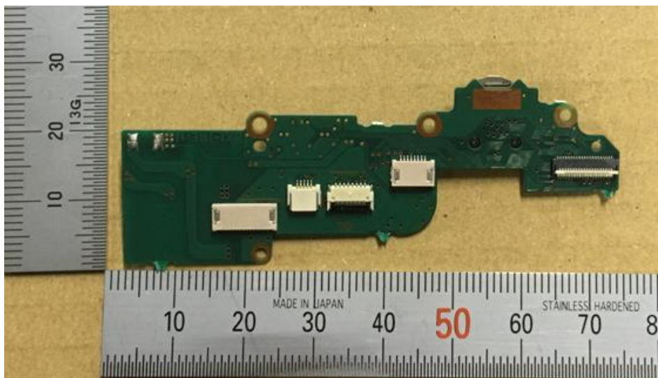
PWBTOP_B
