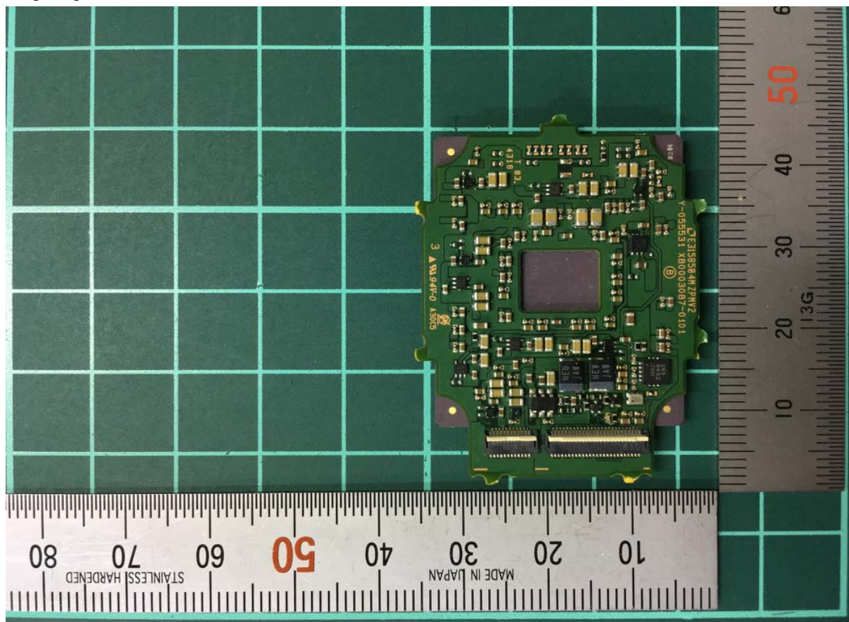
PWB_CMOS_B
