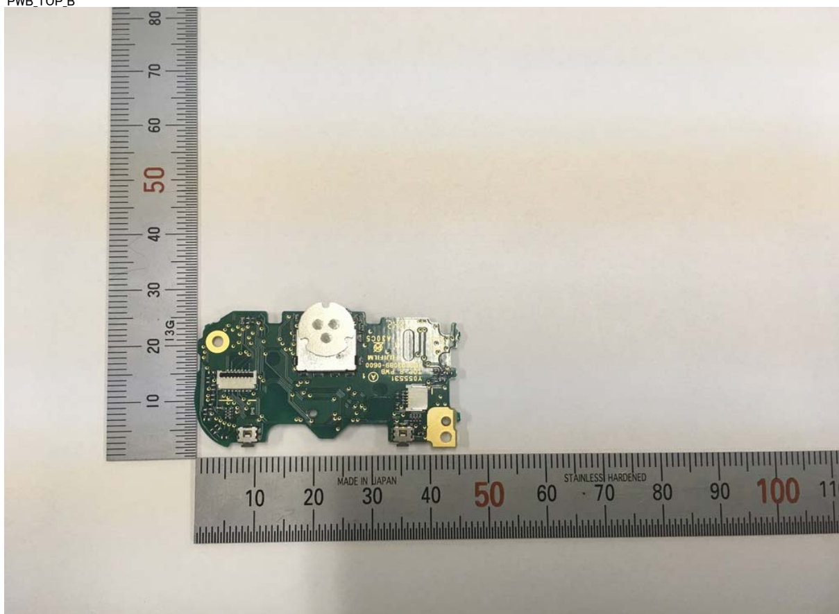
PWB_TOP.B
