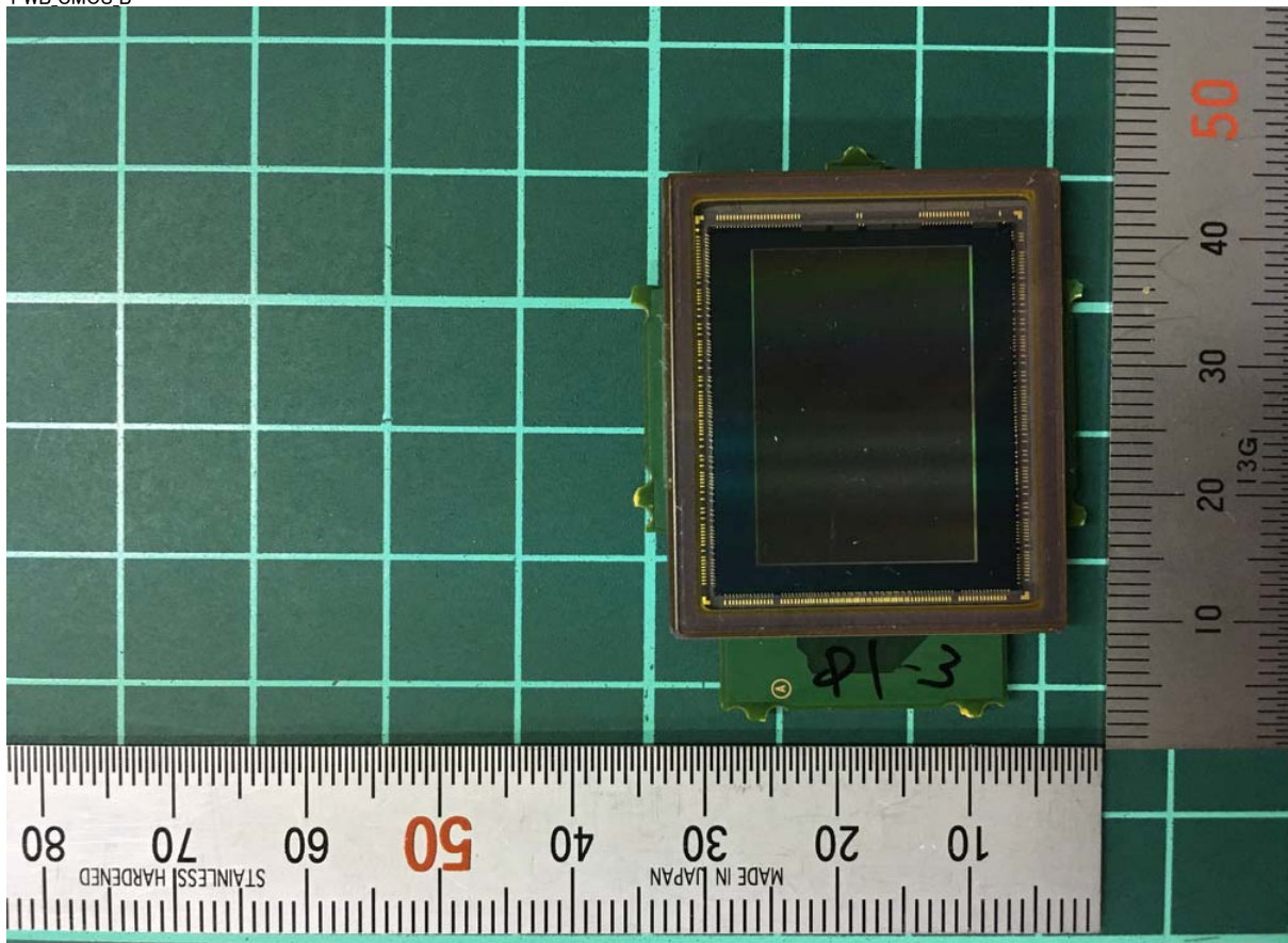
PWB_CMOS_B
