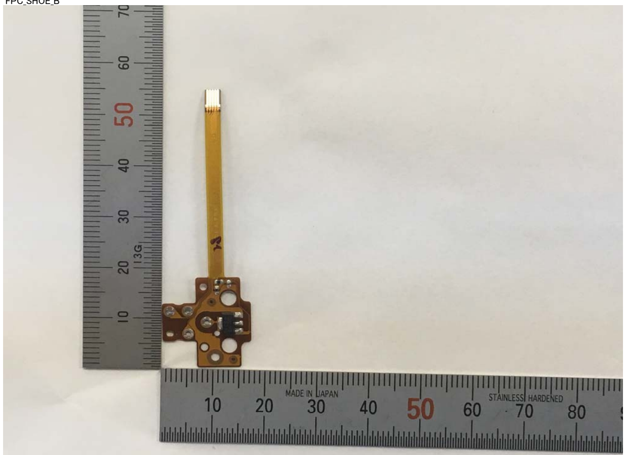
FPC SHOE_B
