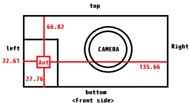
Fig.7 Antenna position (Front side)
