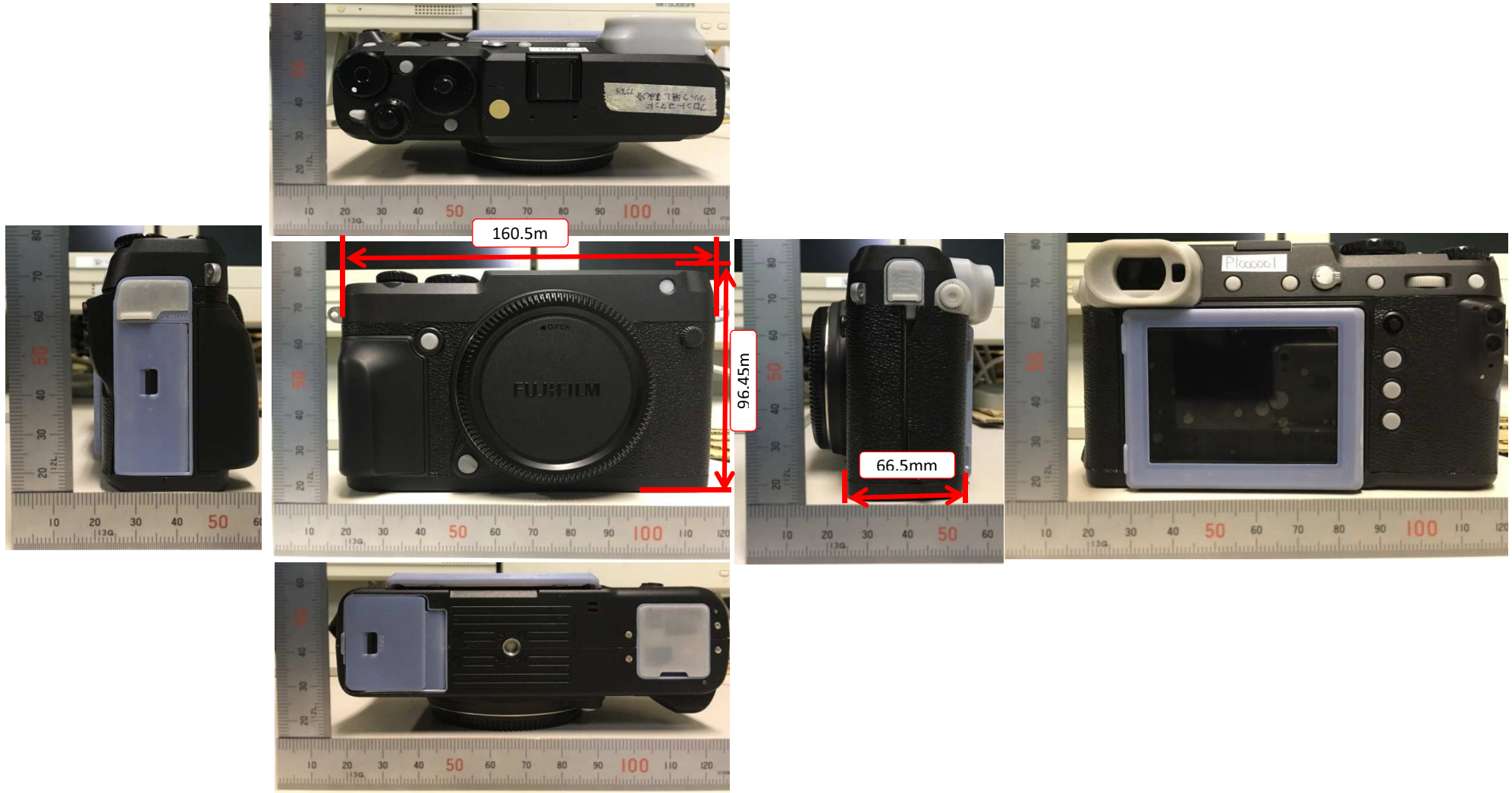
Y-054861 Figure of external form dimensions
