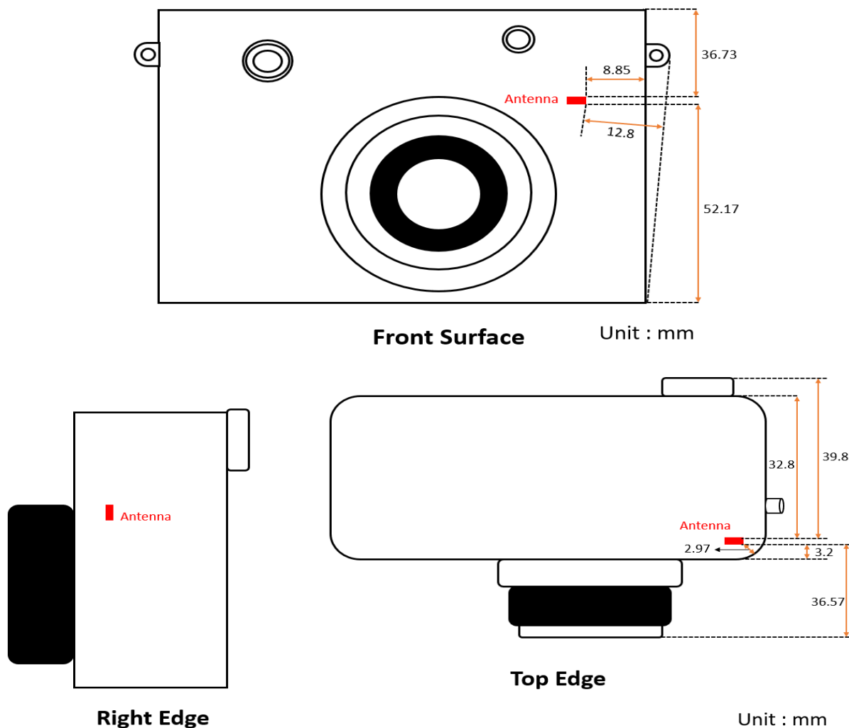
Photograph 15. Antenna position of EUT
