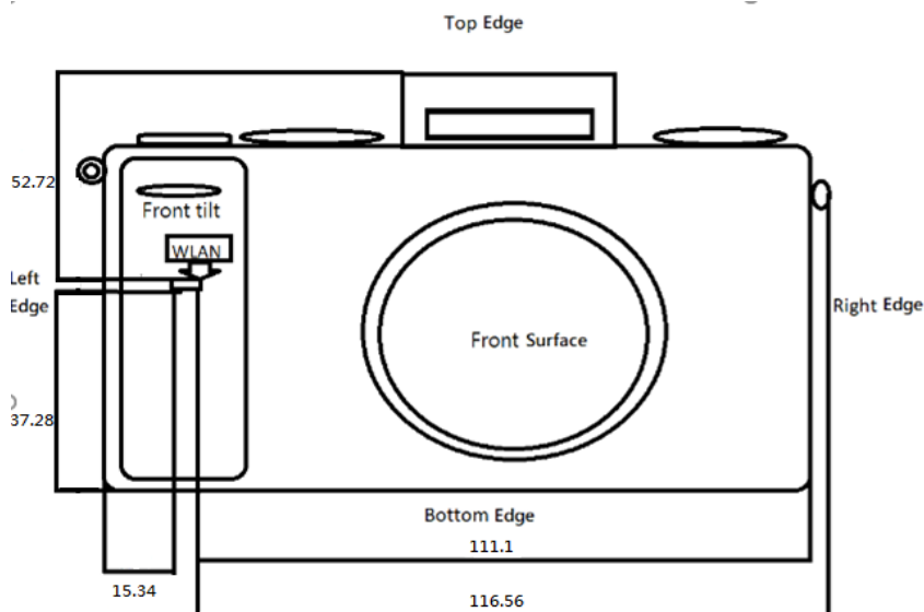
Photograph 7. Antenna position of EUT (Front view)
