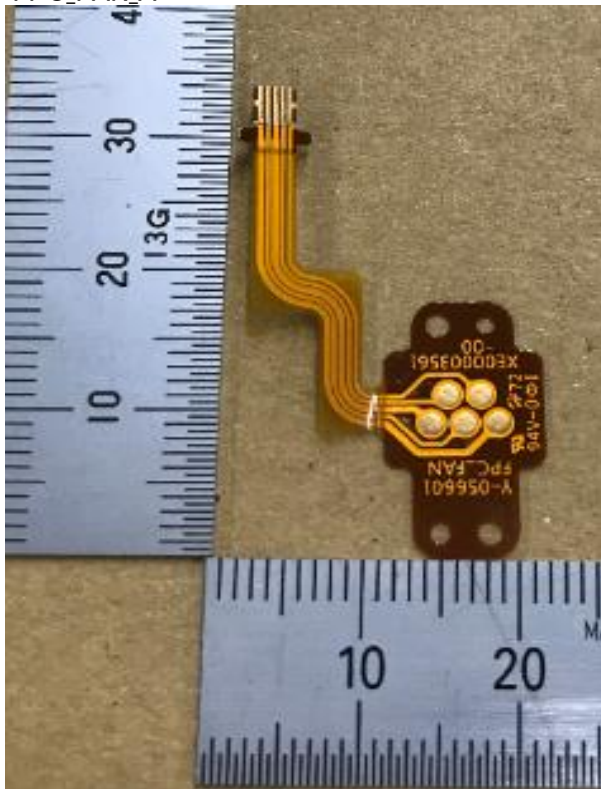
FPC_FAN_A
