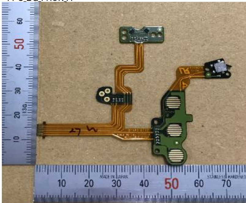
FPC_BG_FRON_A
