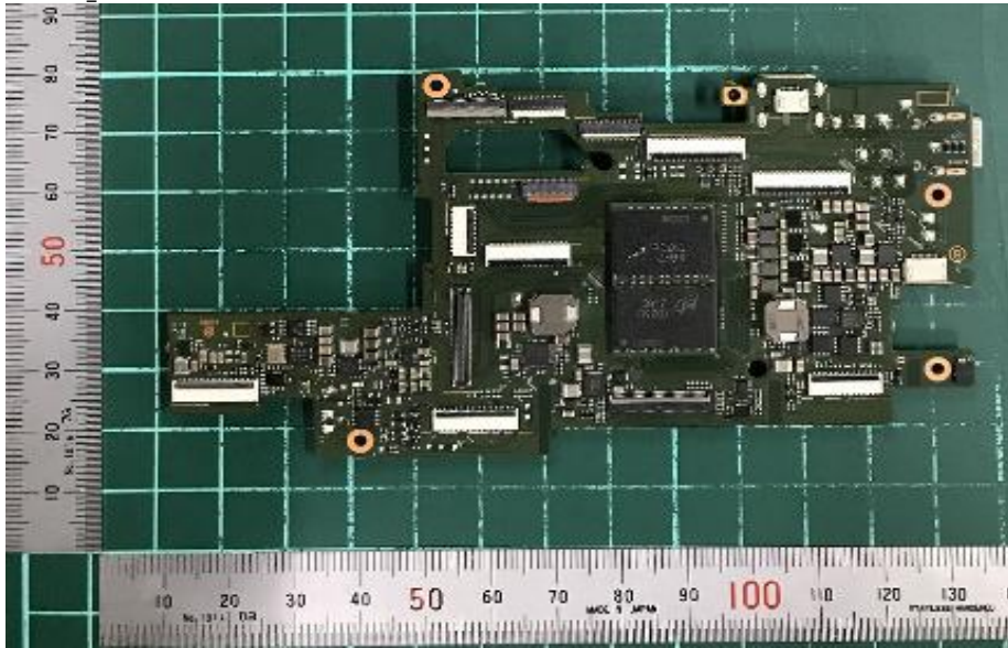
MAIN A
