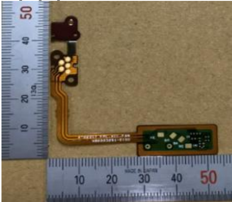
FPC_ACC_FAN_A
