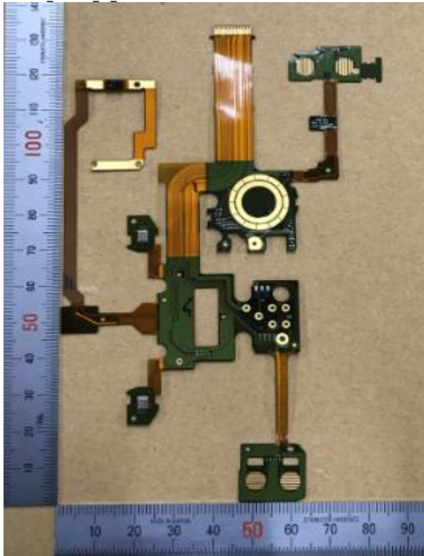
FPC_TOP_L_A
