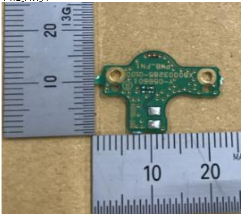
PWB_FN1_A
