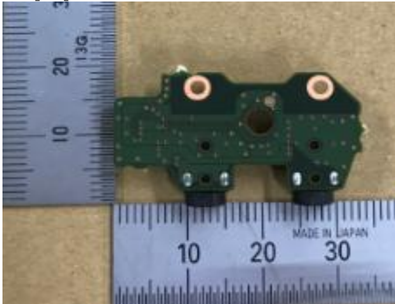
PWB_MIC_A
