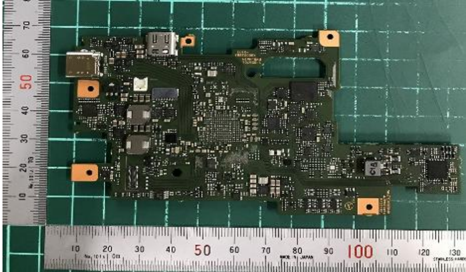
MAIN B
