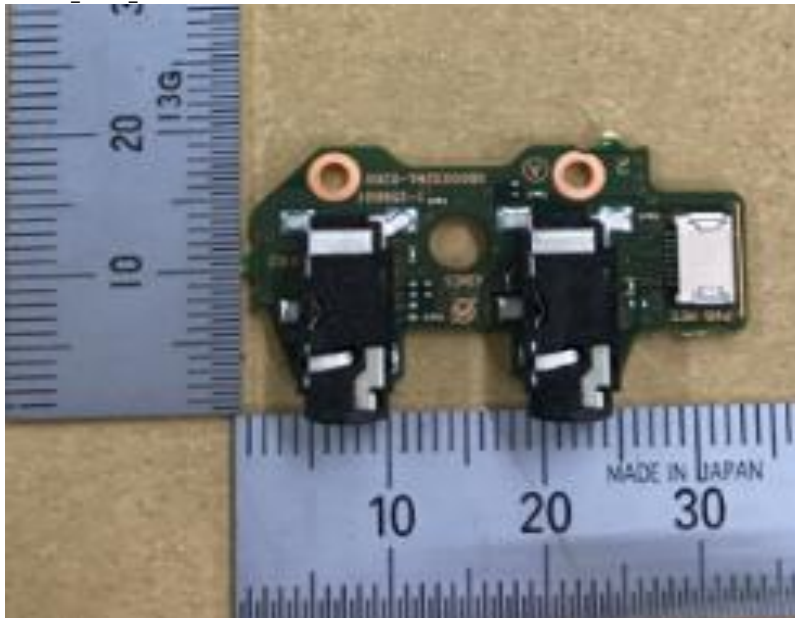
PWB_MIC_B
