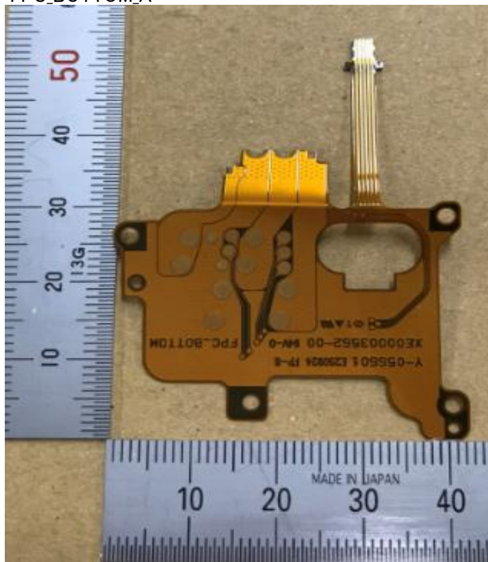
FPC_BOTTOM_A
