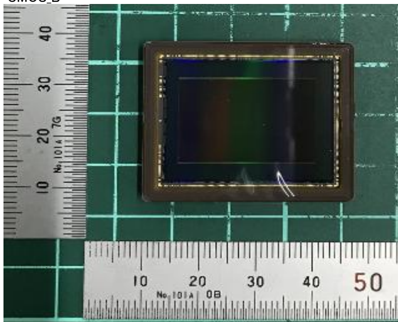
CMOS_B
