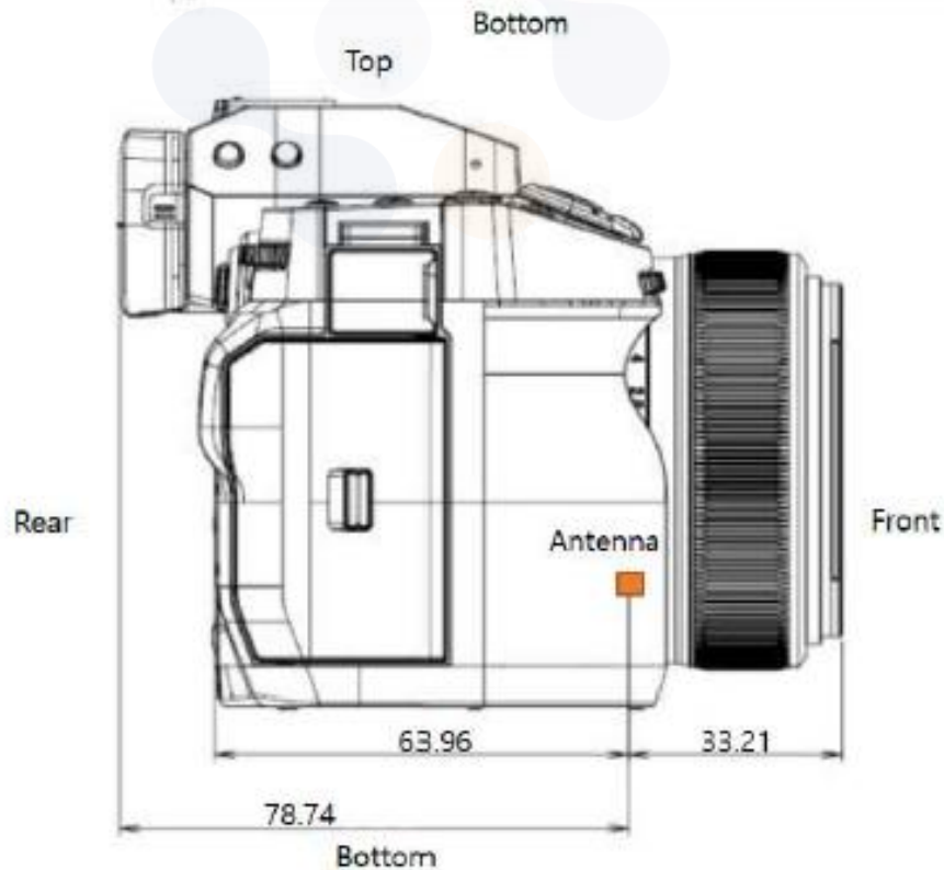
Right view
