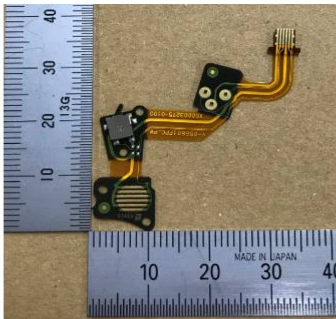
FPC_PW_A
