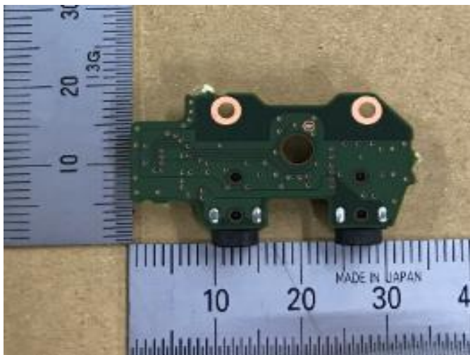
PWB_MIC_B
