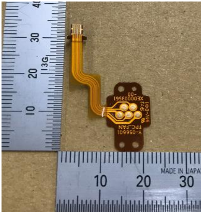
FPC_FAN_A
