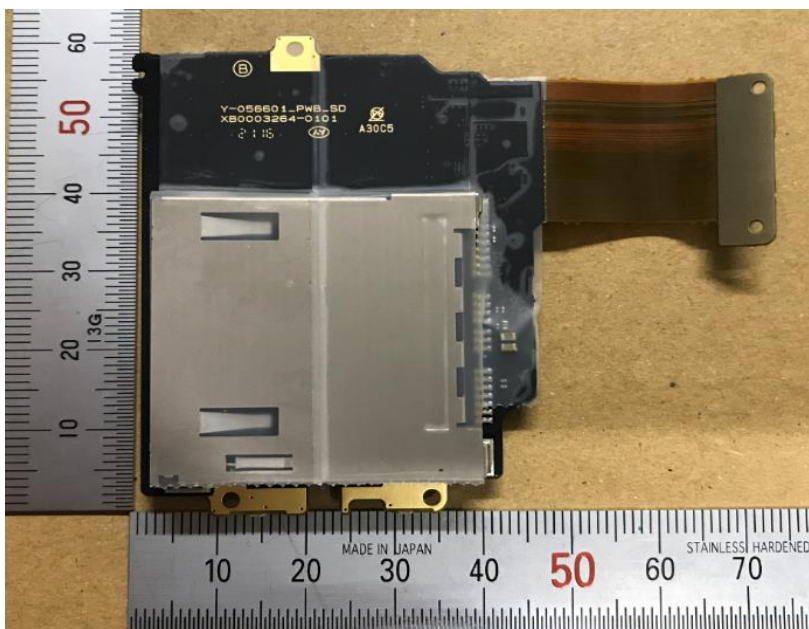
PWB_SD_B
