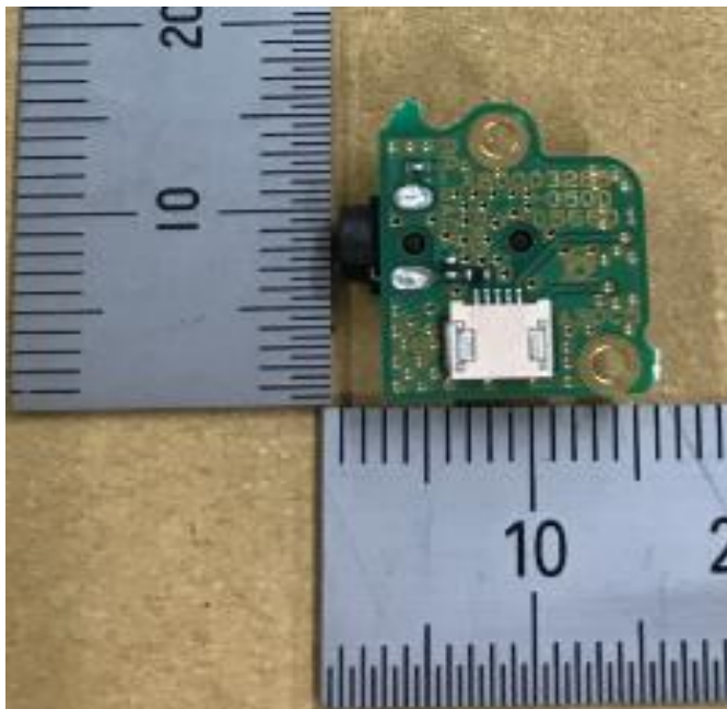
PWB_RR_JACK_A
