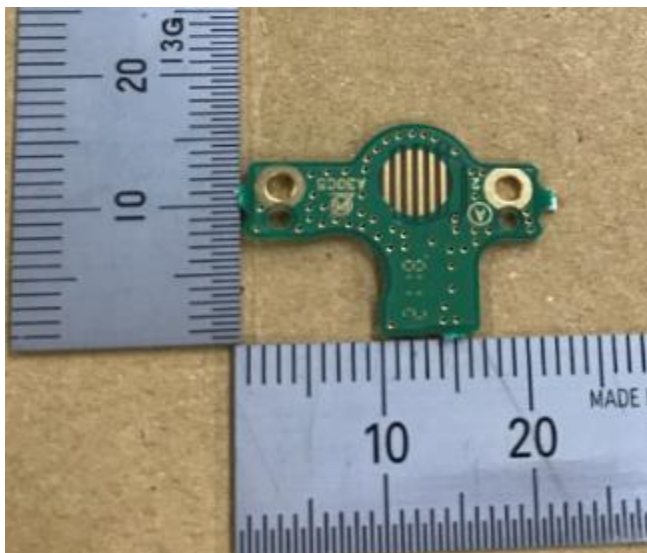
PWB_FN1_B
