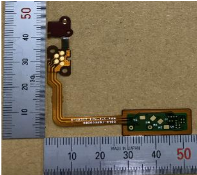
FPC_ACC_FAN_A
