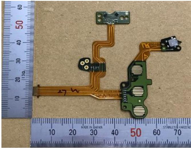
FPC_BG_FRON_A
