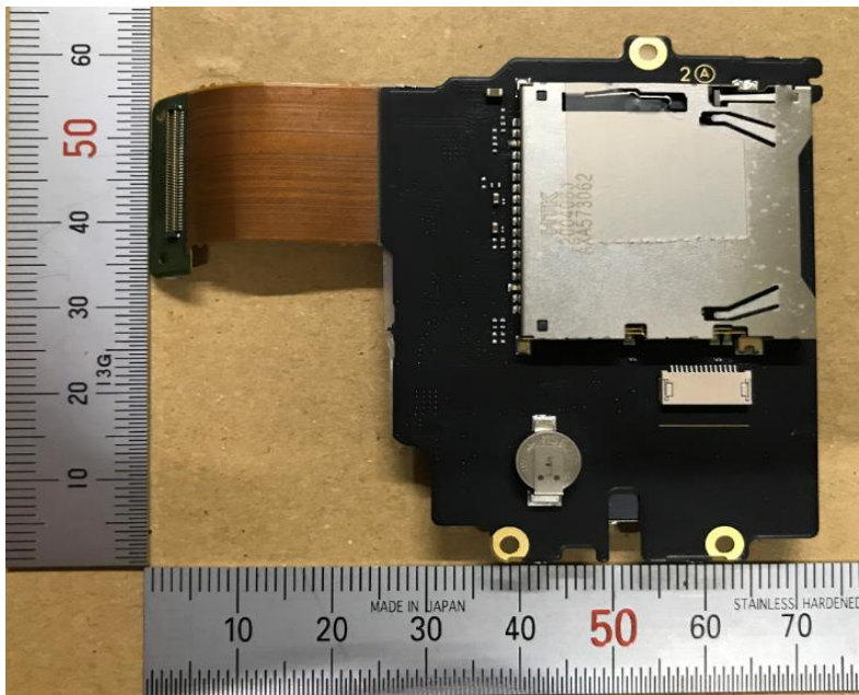
PWB_SD_A
