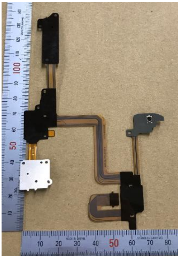
FPC_BG_REAR_B
