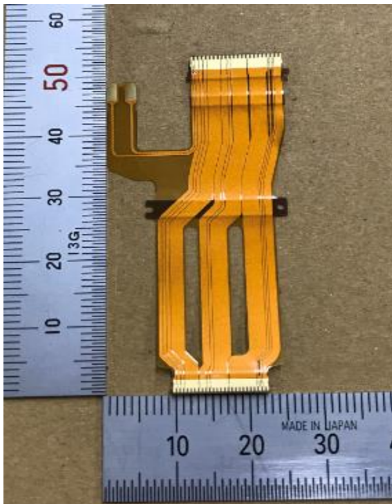
FPC_CAM_PW_B
