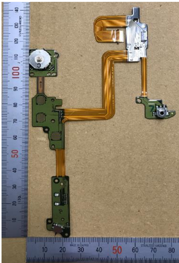
FPC_BG_REAR_B
