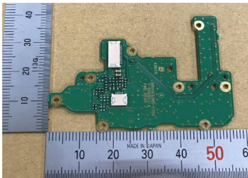
PWB_REAR_B
