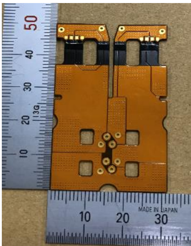
SW-9 294V-0_A
