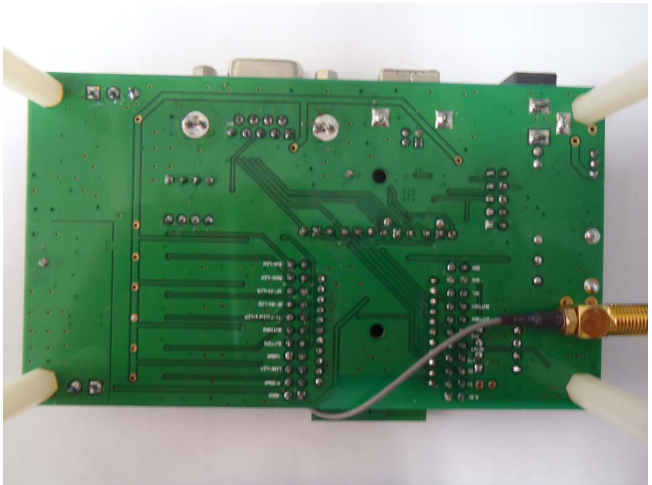
Bottom View of Test Board
