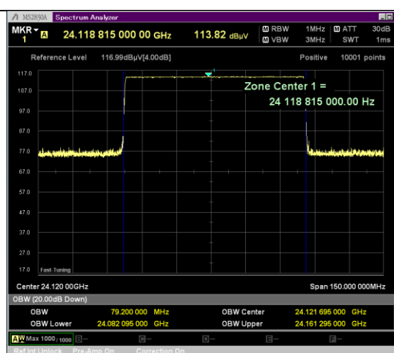
20dB Bandwidth-Mid
