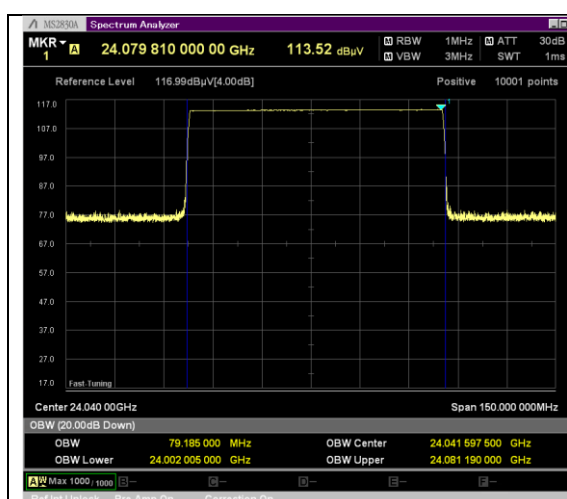
20dB Bandwidth-Low
