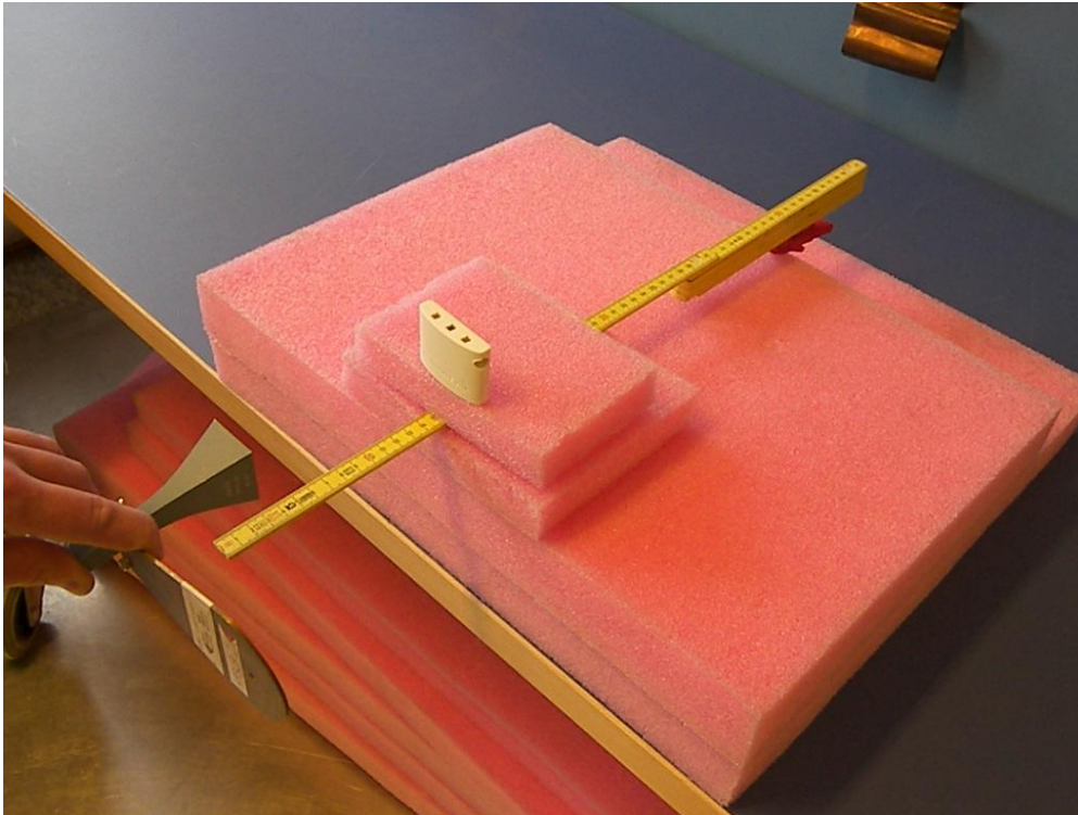
Photo Error! No text of specified style in document.. 10 Test setup regarding radiated emission, spurious, 18-25 GHz.
