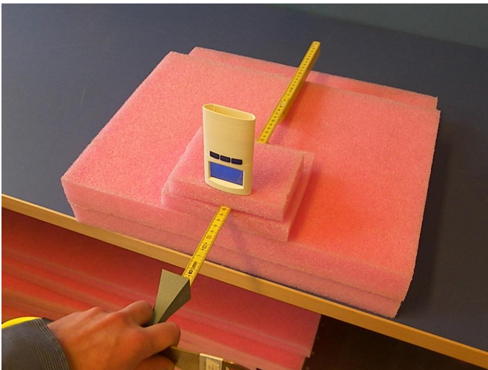
Photo Error! No text of specified style in document.. 11 Test setup regarding radiated emission, spurious, 18-25 GHz.
