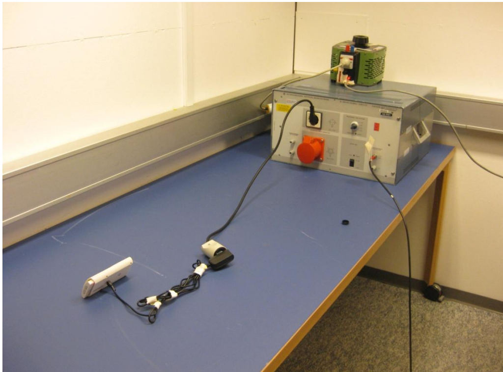
Photo Error! No text of specified style in document..1 Test setup regarding conducted emission, AC mains.
