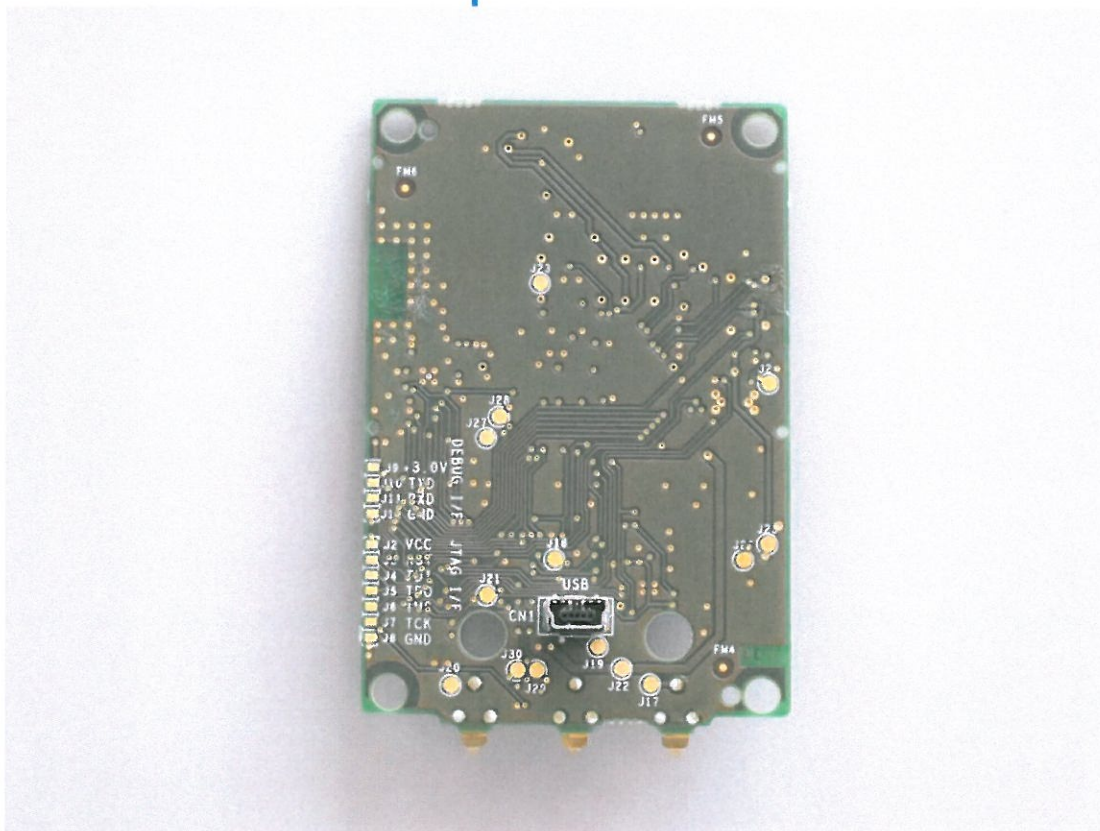
Figure 3 GrindDock - PCB bottom side
