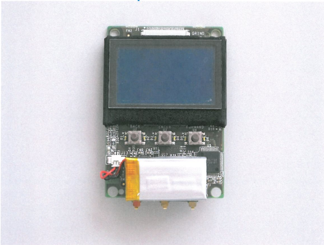
Figure 1 GrindDock - electronics
