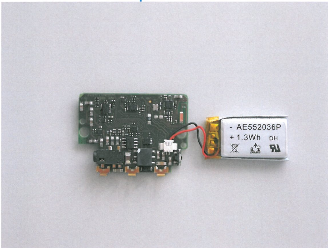
Figure 5 Stimulator – electronics - PCB top side
