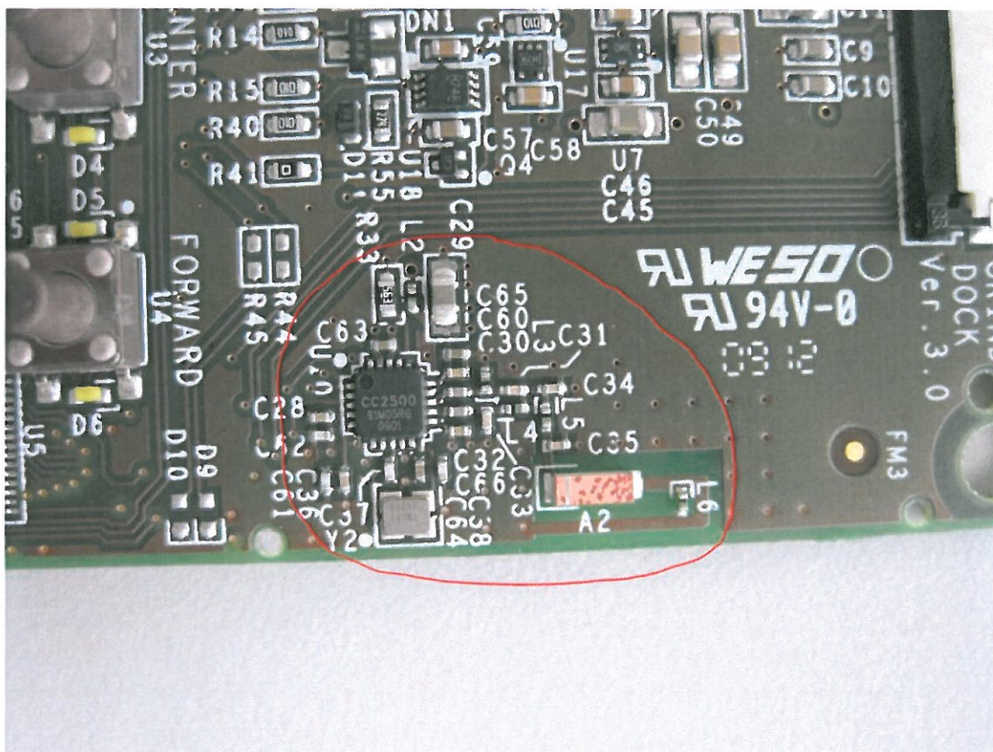
Figure 4 GrindDock - RF circuit (A2 is chip antenna)
