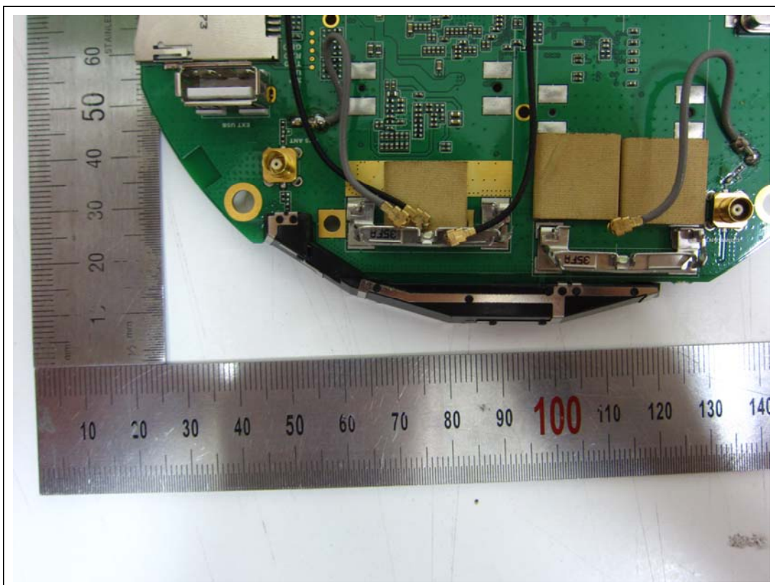
<Internal ANTENNA>
