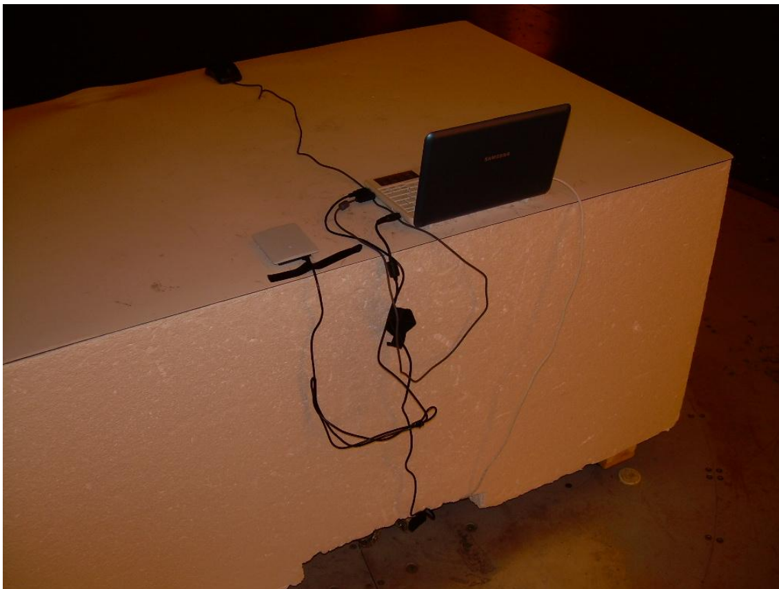
Back View Radiated Emission Setup – Horizontal Placement
