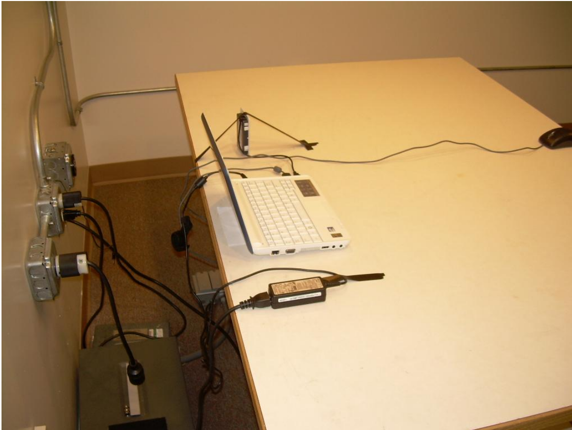
Back View Conducted Emission Setup
