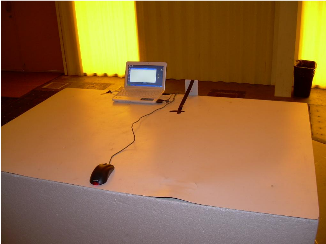
Front View Radiated Test Setup - Vertical EUT Placement
