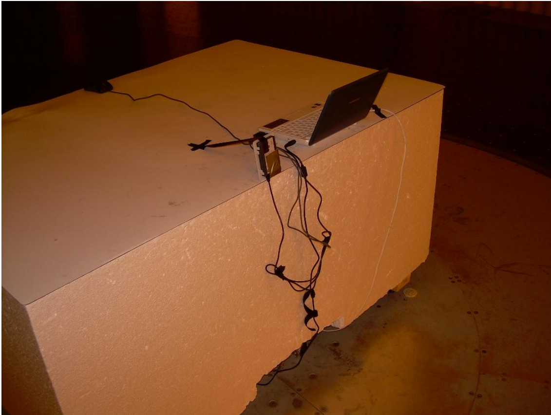
Back View Radiated Test Setup - Vertical EUT Placement
