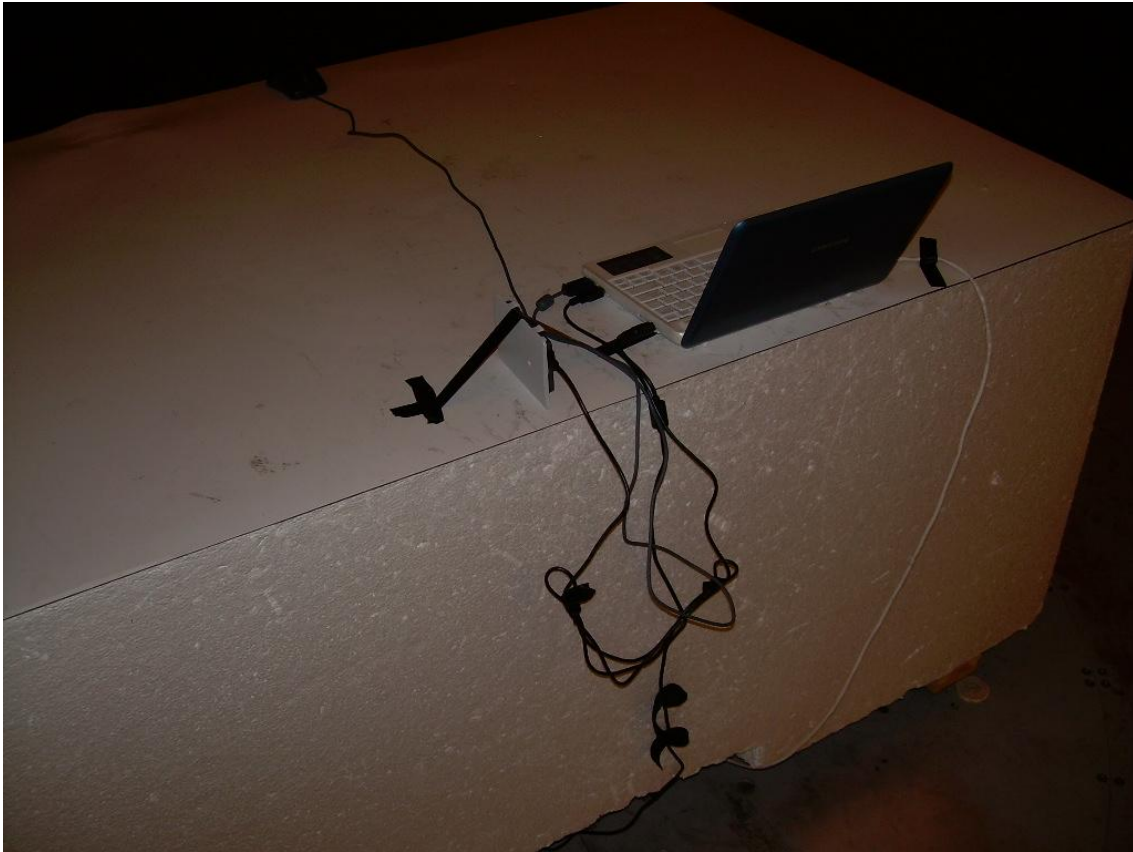
Back View Radiated Test Setup – On-Edge EUT Placement
