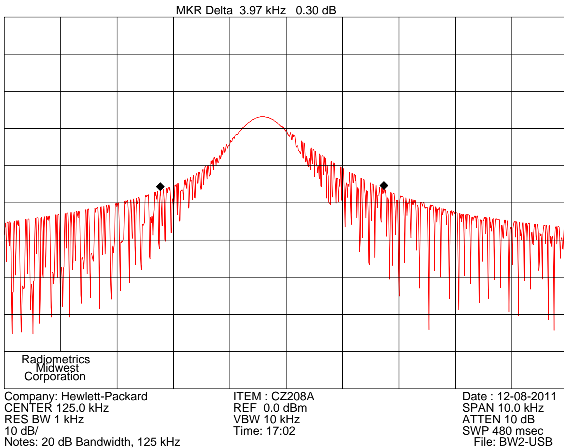
Figure 4. Occupied Bandwidth Plots 125 kHz
