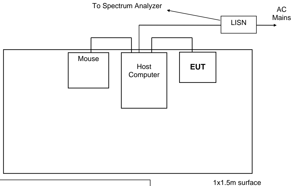
Figure 2. Conducted Emissions Test Setup (Serial Reader)
