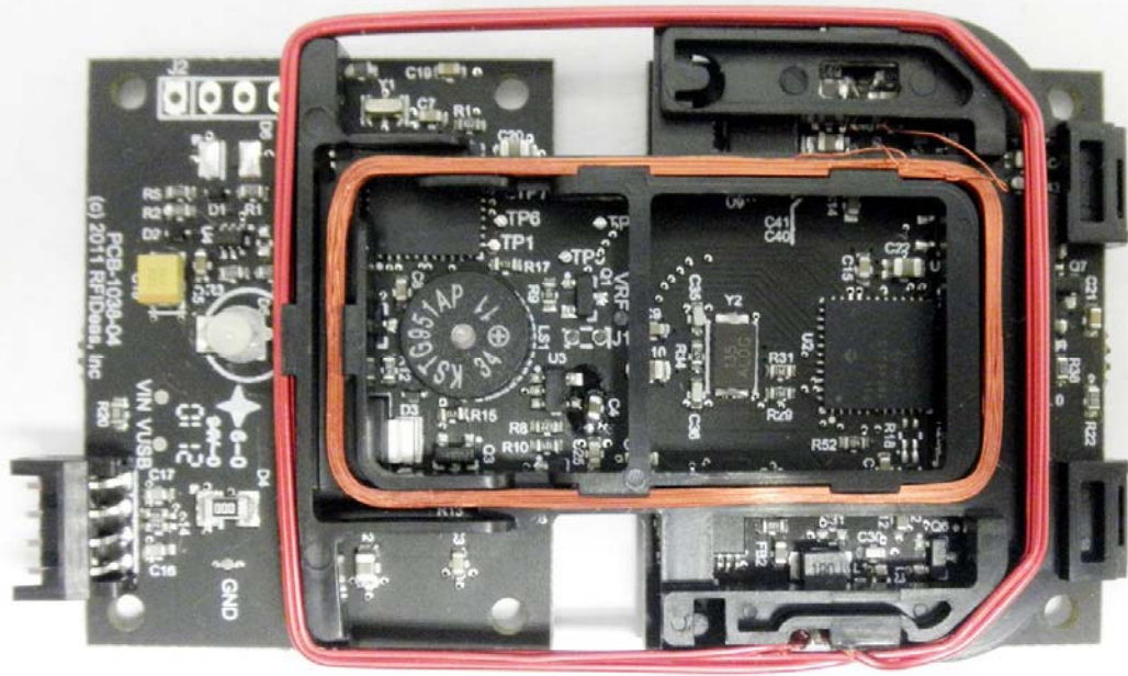
CZ208A - USB reader (Top view PCB Assembly)
