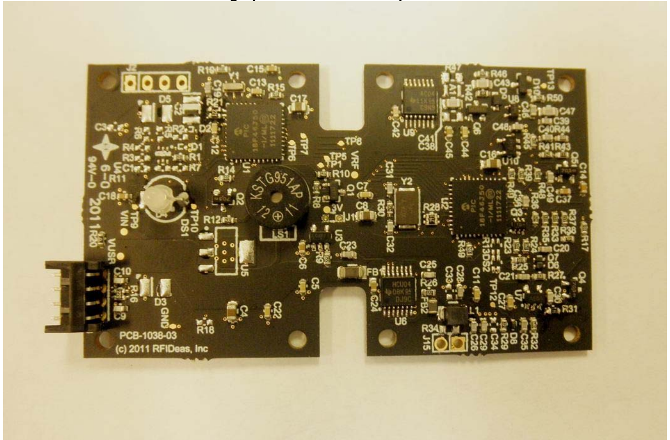
Photograph of PC Board: Component Side
