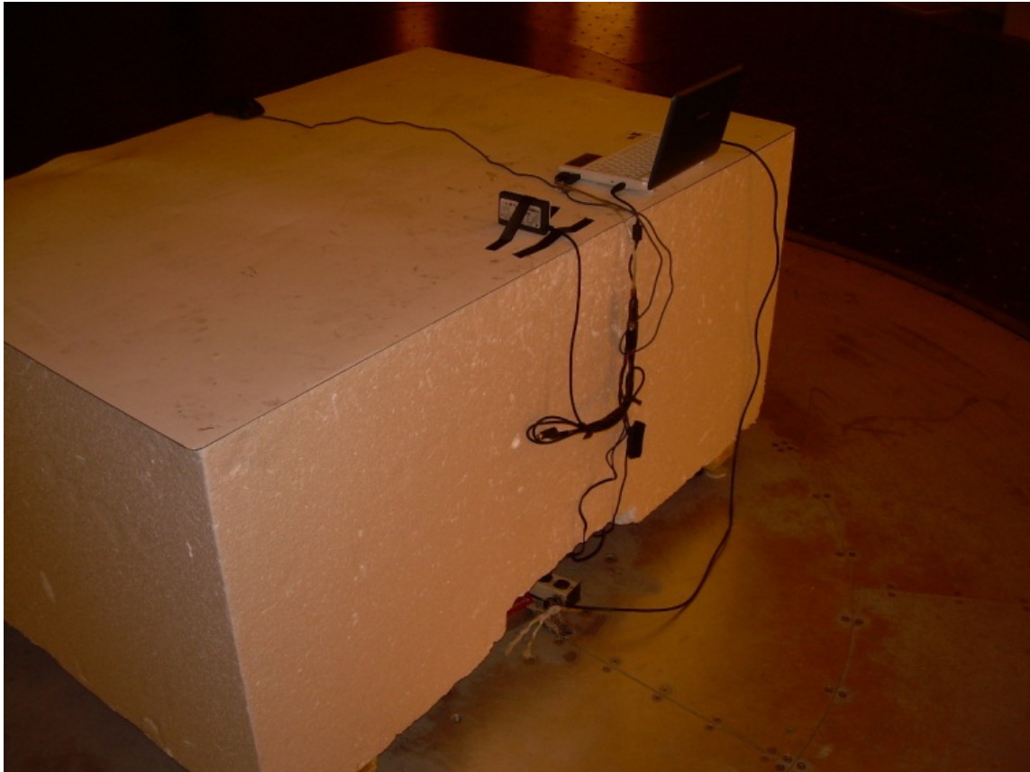
Photograph 4 – View of Radiated Disturbance – EUT On Edge Placement
