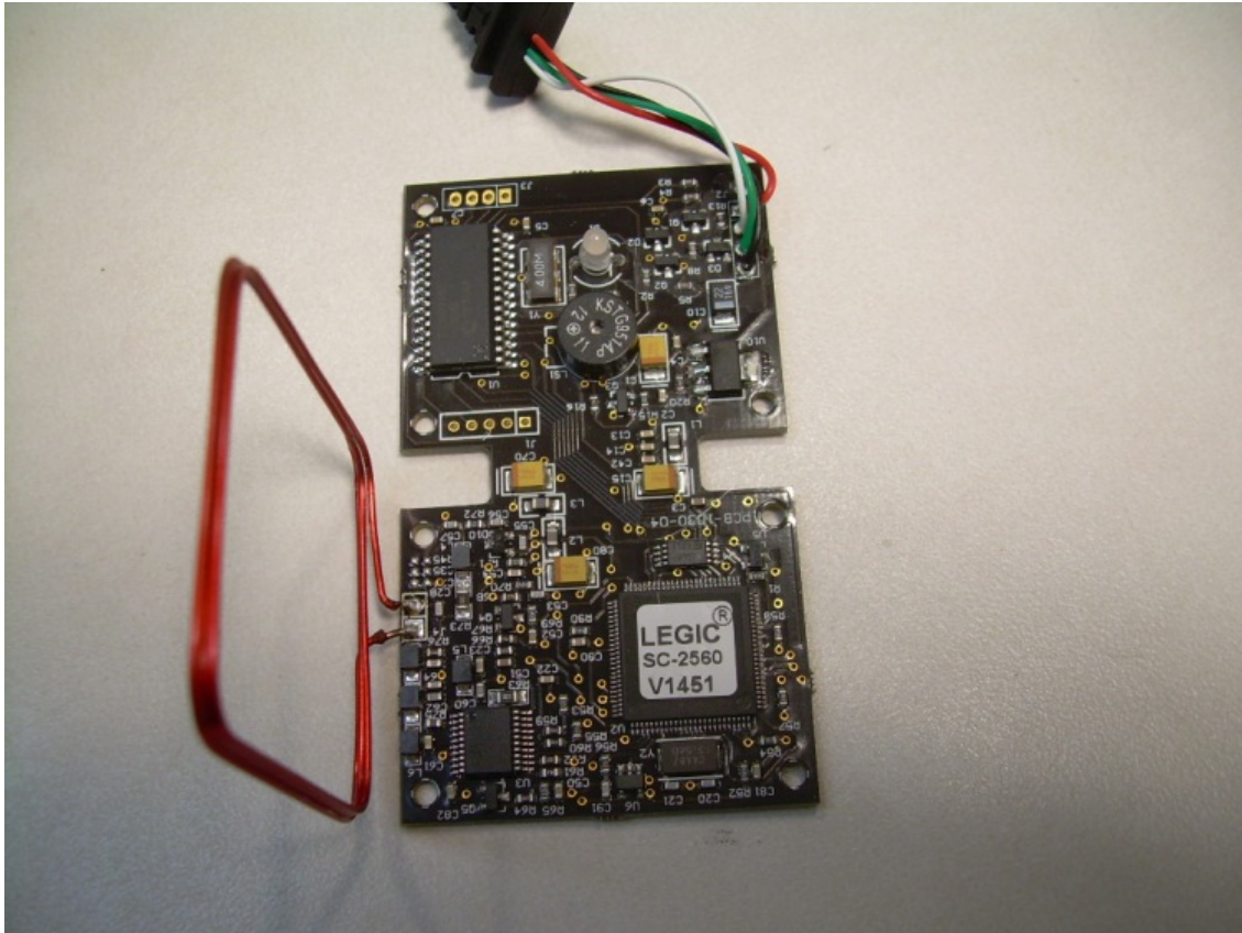
View of the Component Side of the PCB with Antenna Moved
