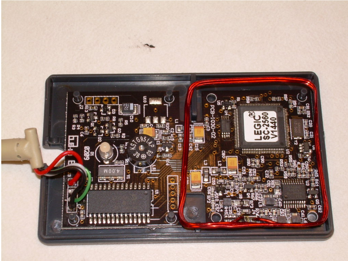
Front Side of the CE984A PCB
