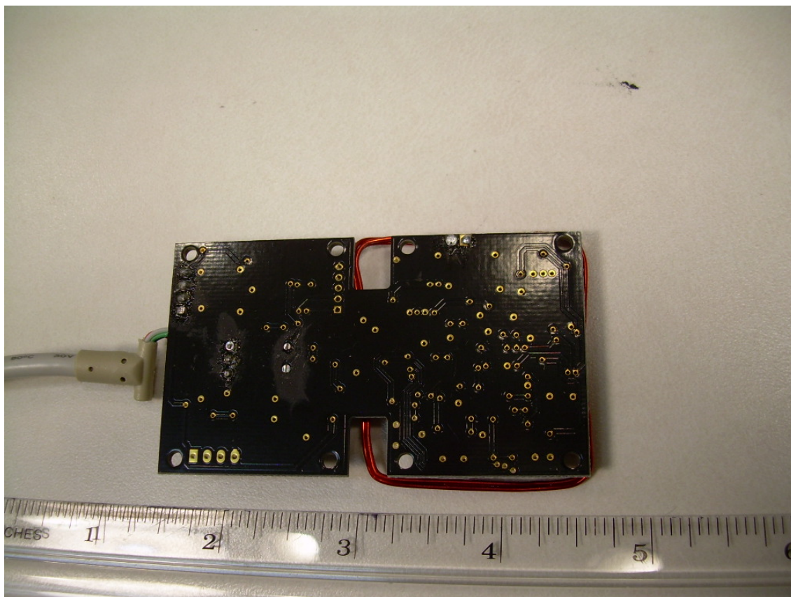
Back Side of the CE984A PCB
