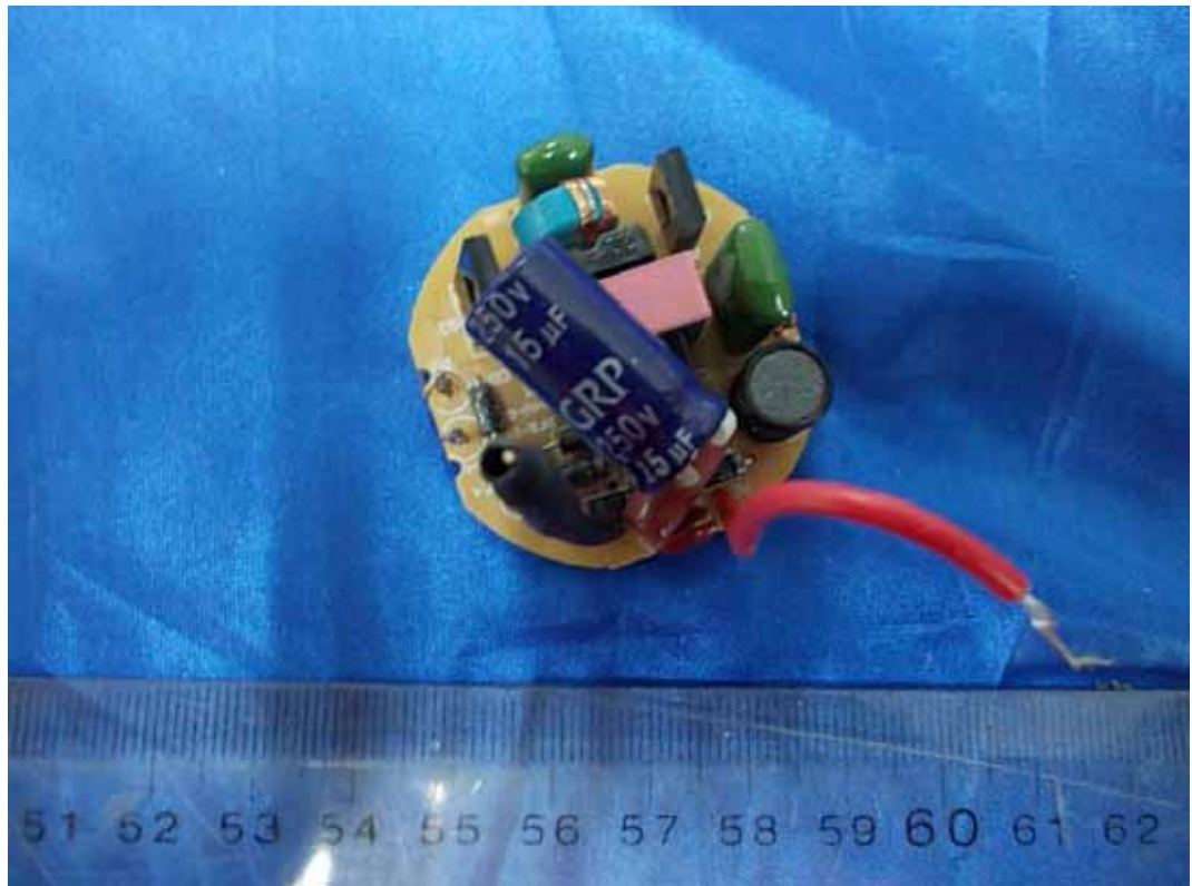
FIGURE 14 FLUORESCENT SELF-BALLASTED LAMPS (M/N: T3 HALF SPIRAL CFL - 18W) MAIN BOARD (COMPONENT SIDE)
