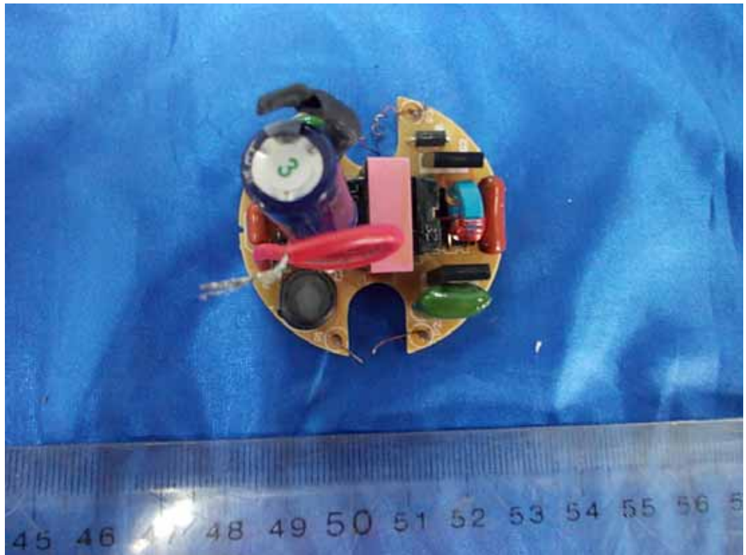
FIGURE 5 FLUORESCENT SELF-BALLASTED LAMPS (M/N: T2 HALF SPIRAL CFL - 18W) MAIN BOARD (COMPONENT SIDE)
