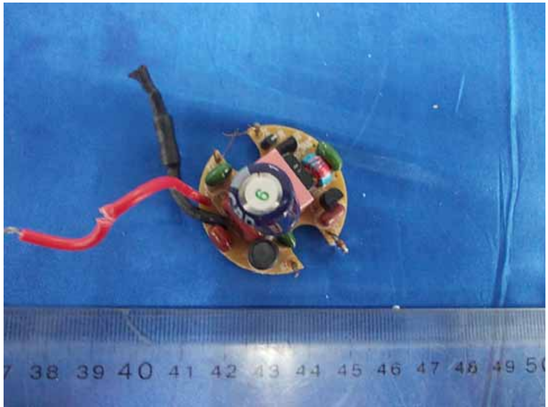
FIGURE 2 FLUORESCENT SELF-BALLASTED LAMPS (M/N: T2 HALF SPIRAL CFL - 13W) MAIN BOARD (COMPONENT SIDE)
