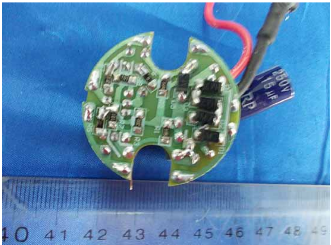
FIGURE 12 FLUORESCENT SELF-BALLASTED LAMPS (M/N: T3 HALF SPIRAL CFL - 13W) MAIN BOARD (SOLDERED SIDE)
