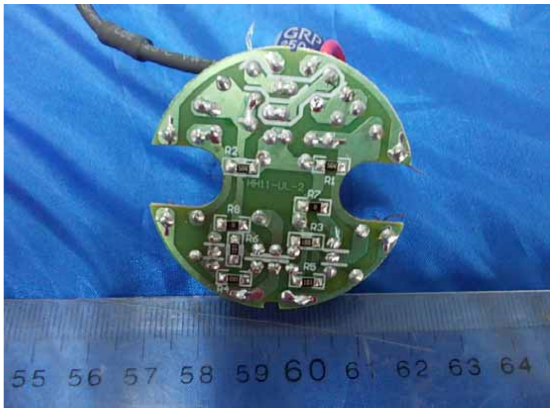
FIGURE 9 FLUORESCENT SELF-BALLASTED LAMPS (M/N: T2 HALF SPIRAL CFL - 23W) MAIN BOARD (SOLDERED SIDE)
