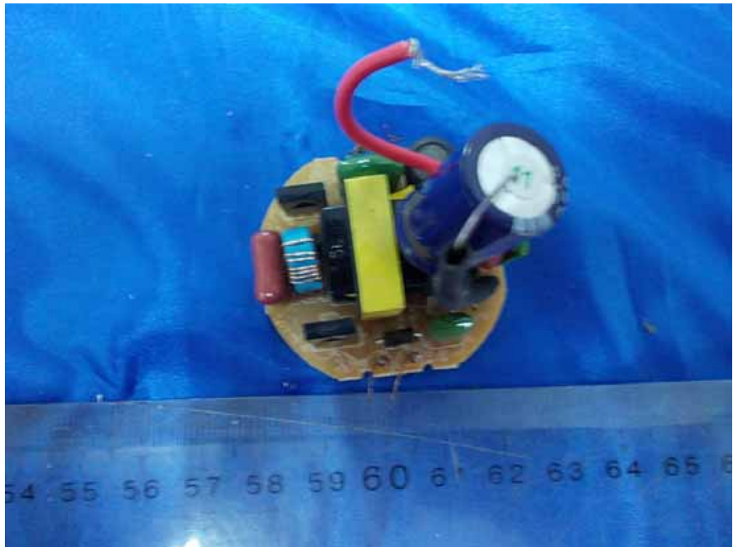
FIGURE 17 FLUORESCENT SELF-BALLASTED LAMPS (M/N: T3 HALF SPIRAL CFL - 23W) MAIN BOARD (COMPONENT SIDE)
