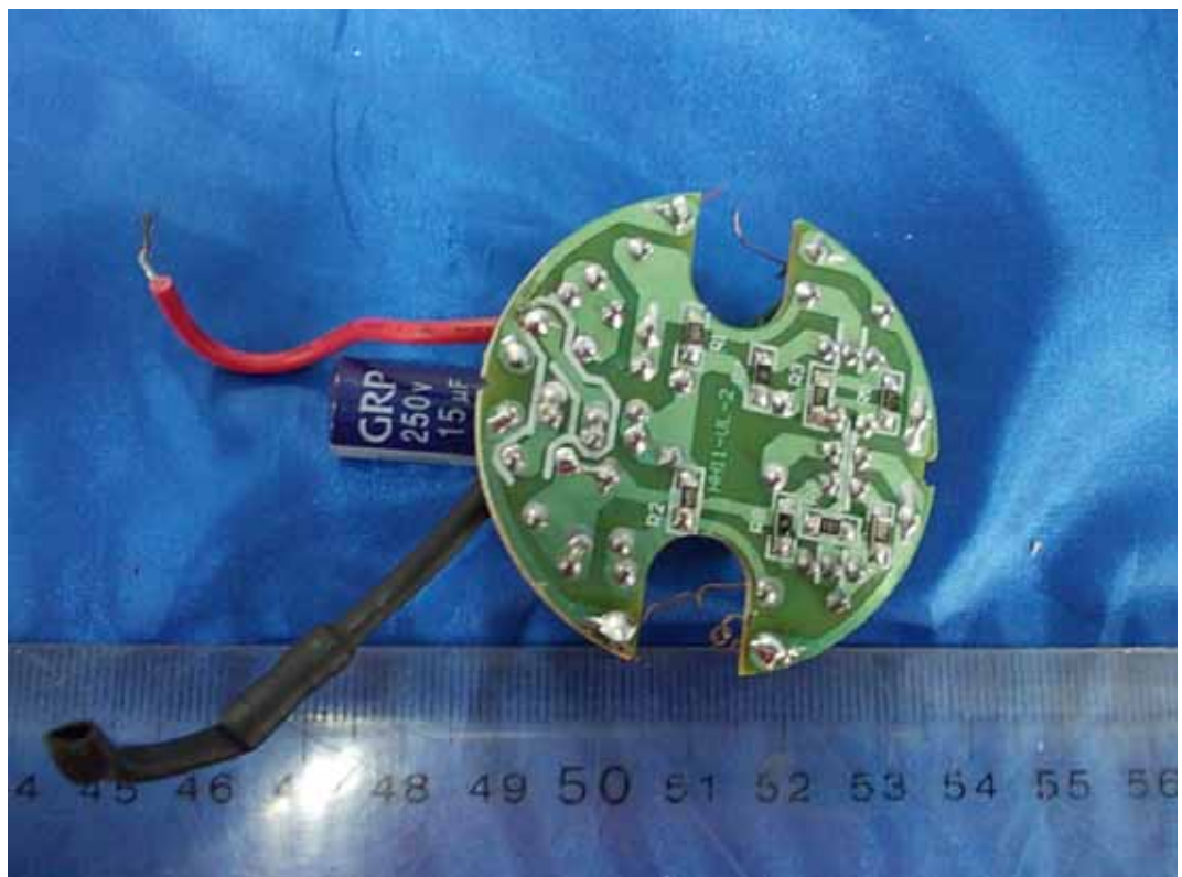
FIGURE 6 FLUORESCENT SELF-BALLASTED LAMPS (M/N: T2 HALF SPIRAL CFL - 18W) MAIN BOARD (SOLDERED SIDE)
