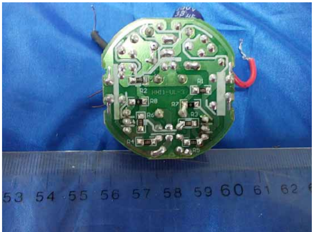
FIGURE 18 FLUORESCENT SELF-BALLASTED LAMPS (M/N: T3 HALF SPIRAL CFL - 23W) MAIN BOARD (SOLDERED SIDE)
