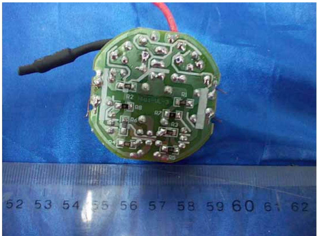
FIGURE 15 FLUORESCENT SELF-BALLASTED LAMPS (M/N: T3 HALF SPIRAL CFL - 18W) MAIN BOARD (SOLDERED SIDE)
