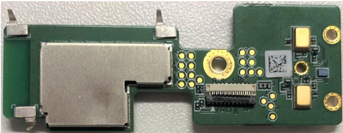
340-26732-000 PCBA, GNSS-Back with shield, SPCC1
