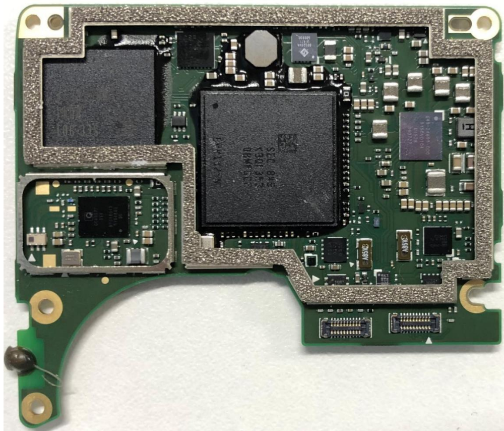
340-26747-001 PCBA MAIN-Front with shield removed, SPCC1
