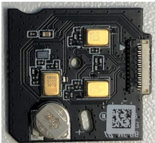
340-27493-000 PCBA, FRONT MICS-Front, SPCC1
