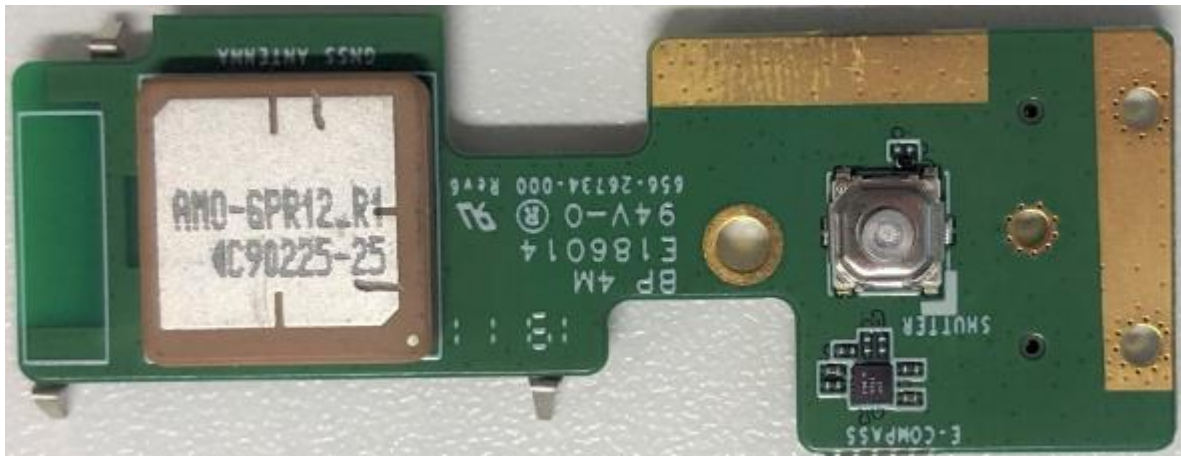
340-26732-000 PCBA, GNSS-Front, SPCC1
