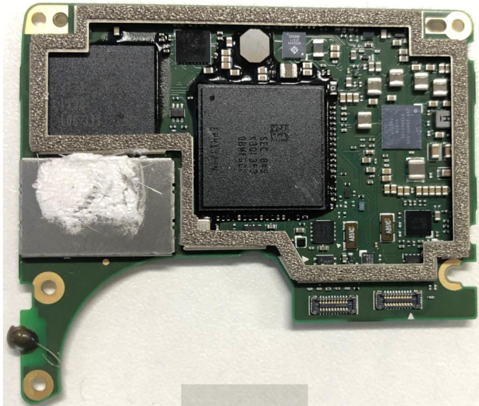
340-26747-001 PCBA MAIN-Front with shield, SPCC1
