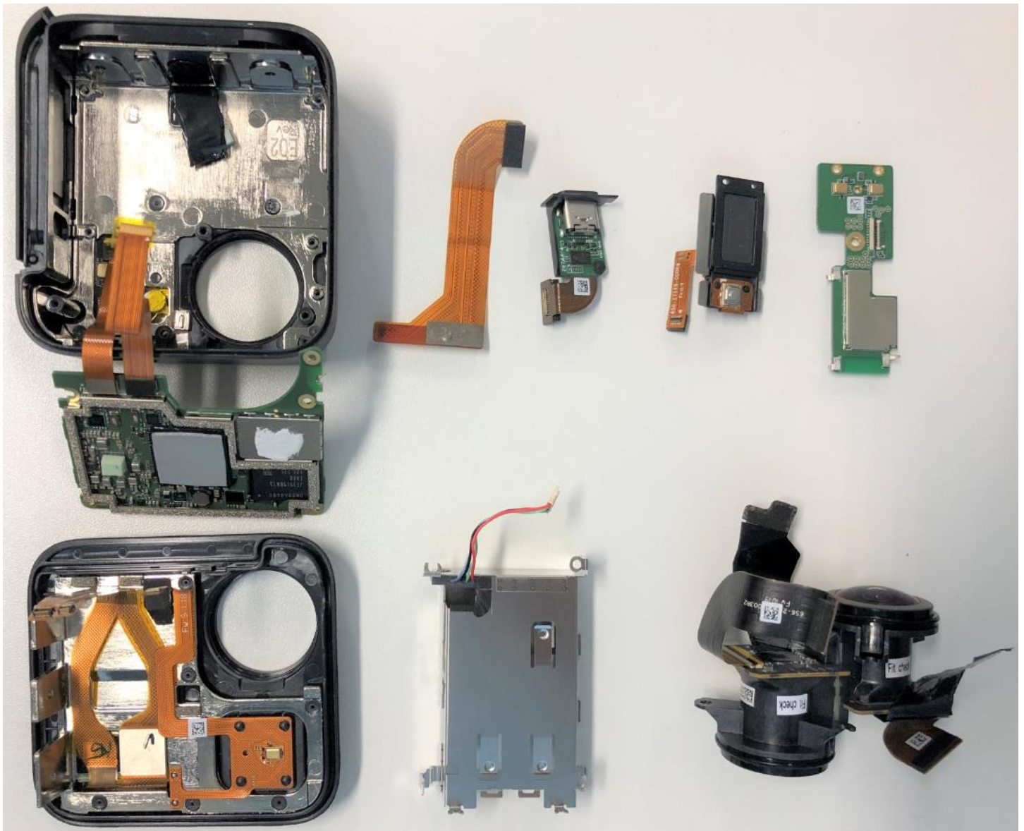
Battery counterpart, Lens module, USB board, FPC, Main board, speaker, GPS board removed, SPCC1
