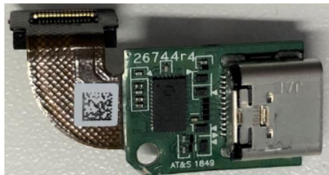
340-26742-000 ASSY, RFPC, USB-C-Front, SPCC1
