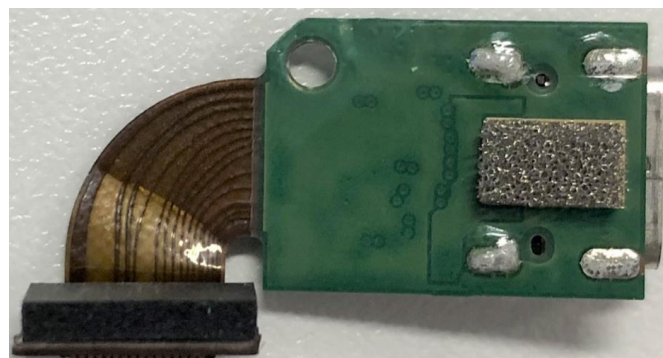
340-26742-000 ASSY, RFPC, USB-C-Back, SPCC1
