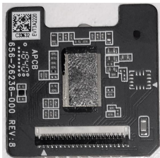
340-26778-000 PCBA, SENSOR BOARD WOUT IMU-Front, SPCC1
