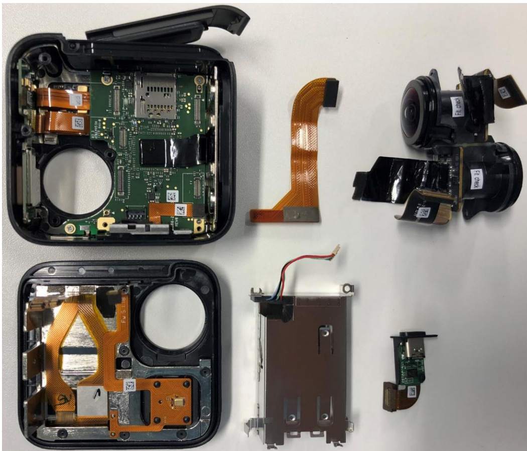
Battery counterpoint, Lens module, USB board and FPC removed, SPCC1
