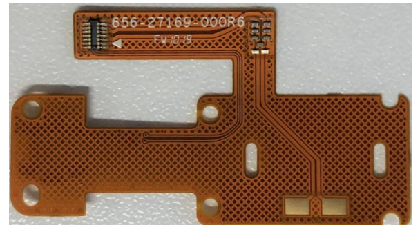
340-27168-000 ASSY, FPC, MODE, SPEAKER-Back, SPCC1
