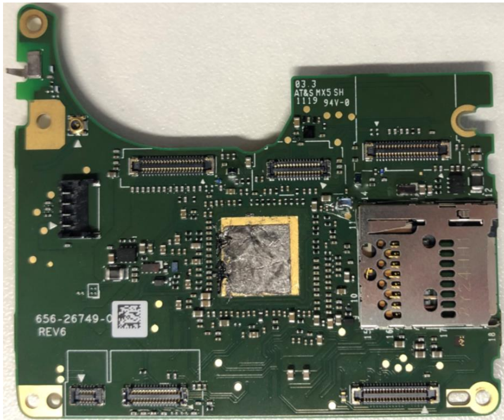
340-26747-001 PCBA MAIN-Back, SPCC1
