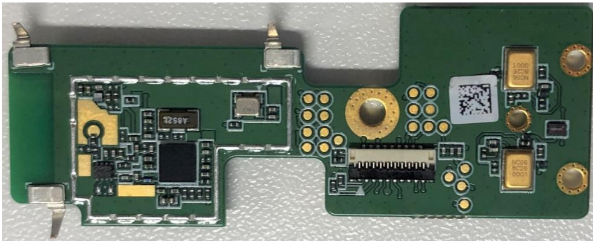
340-26732-000 PCBA, GNSS-Back with shield removed, SPCC1
