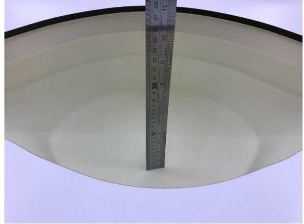
Liquid depth in the Flat of SAM1 phantom(Body)
