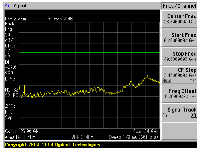
Middle Channel 5610 MHz (6GHz – 40GHz)
