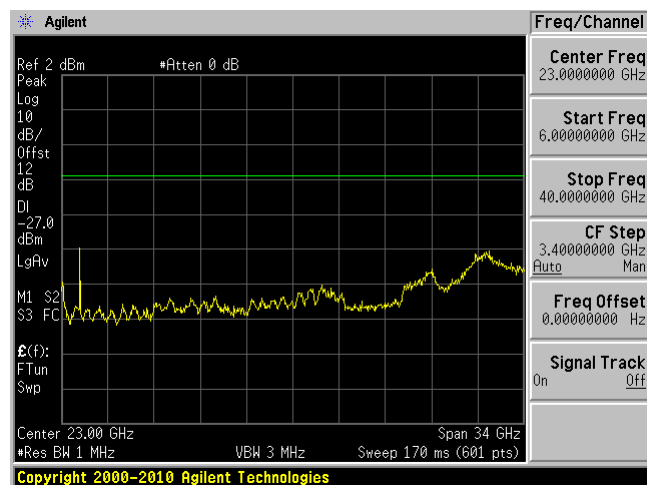
Low Channel 5530 MHz (6GHz – 40GHz)
