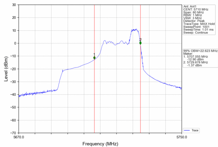
802.11ax(HEW40) HCH 5710MHz RU106_56 Ant1 NTNv
