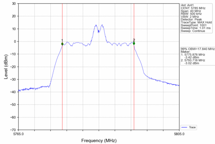
802.11ax(HEW20) MCH 5785MHz RU52_38 Ant1 NTNv
