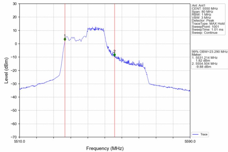
802.11ax(HEW40)_MCH_5550MHz_RU242_61_Ant1_NTNV
