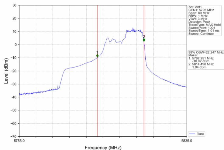
802.11ax(HEW40) HCH 5795MHz RU242_62_Ant1_NTNV
