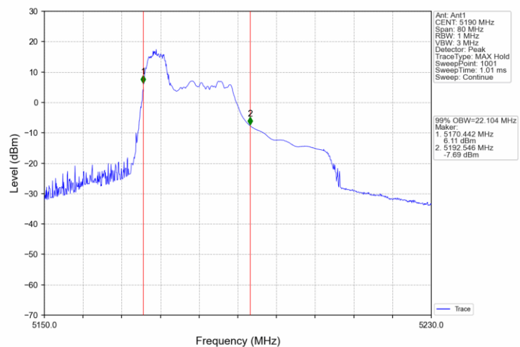
802.11ax(HEW40) LCH 5190MHz RU106 53 Ant1 NTNv
