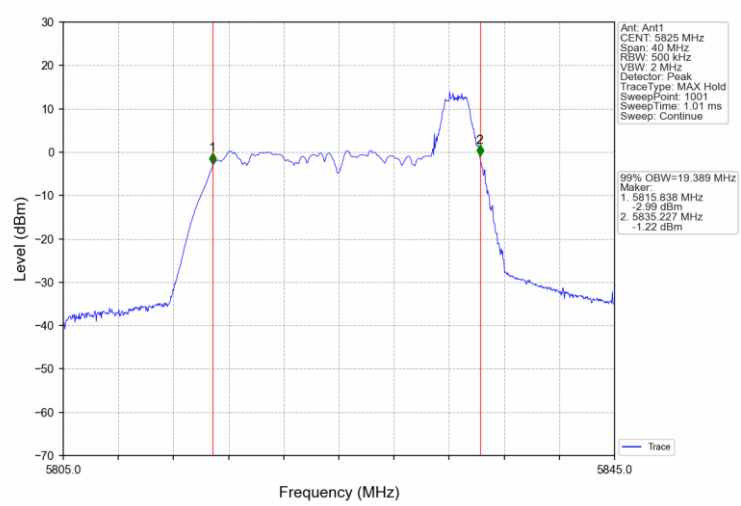
802.11ax(HEW20)_HCH_5825MHz_RU52_40_Ant1_NTNV
