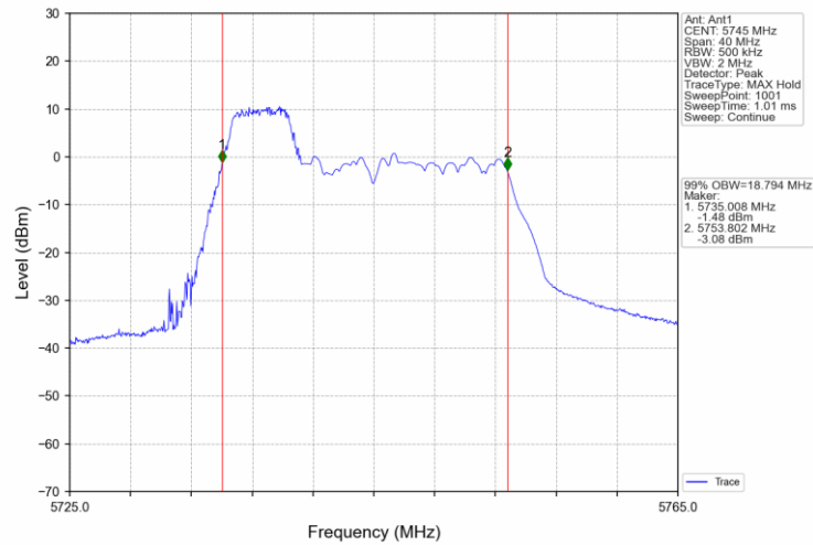
802.11ax(HEW20) LCH 5745MHz RU106_53 Ant1 NTNv
