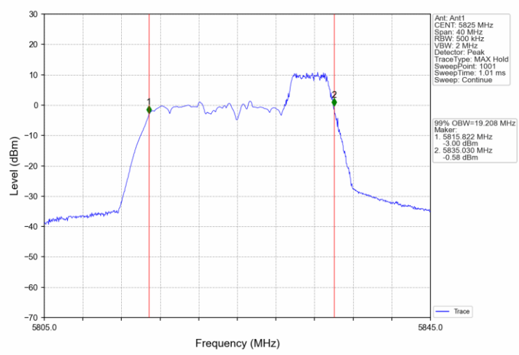
802.11ax(HEW20)_HCH_5825MHz_RU106_54_Ant1_NTNV
