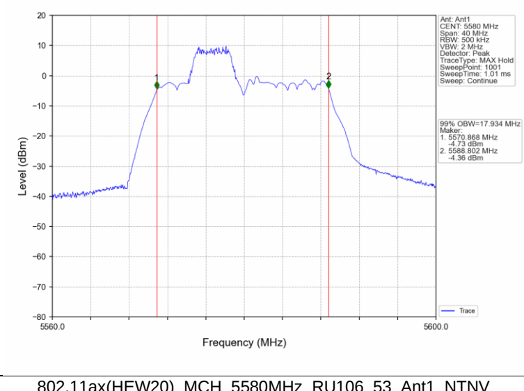
802.11ax(HEW20) MCH 5580MHz RU106_53 Ant1 NTNv
