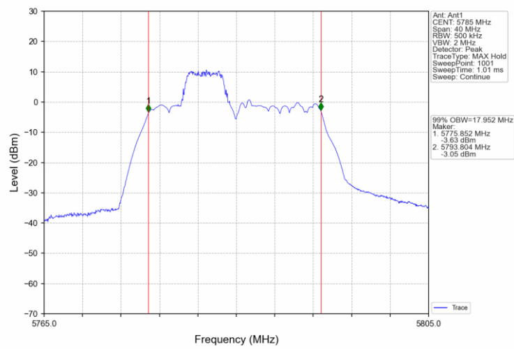
802.11ax(HEW20) MCH 5785MHz RU106_53 Ant1 NTNv
