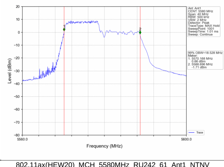
802.11ax(HEW20) MCH 5580MHz RU242_61 Ant1 NTNv
