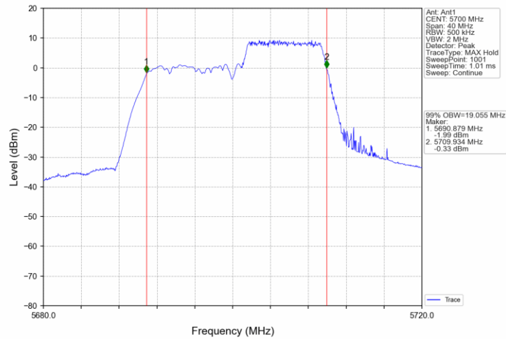
802.11ax(HEW20)_HCH_5700MHz_RU242_61_Ant1_NTNV
