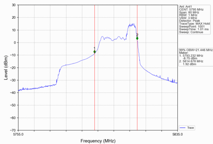
802.11ax(HEW40) HCH 5795MHz RU106 56 Ant1 NTNv
