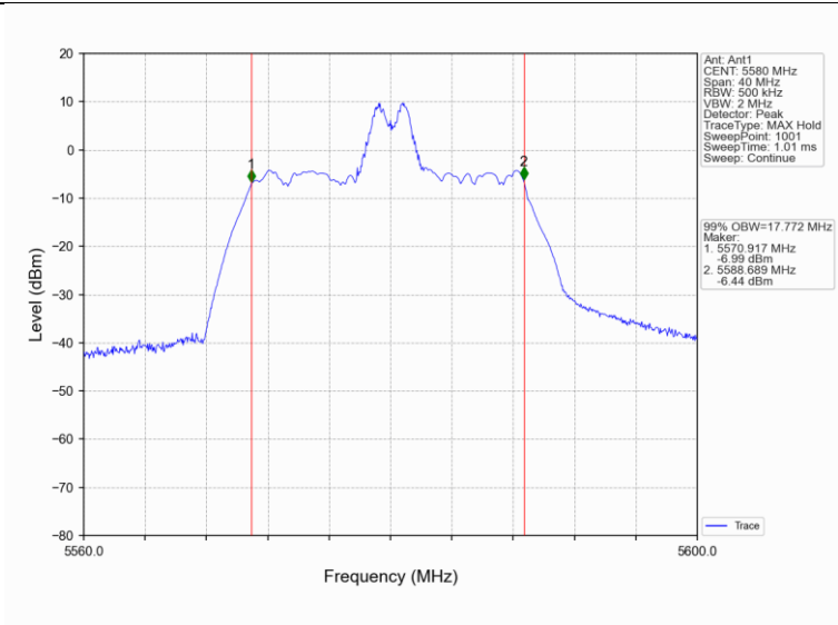
802.11ax(HEW20) MCH 5580MHz RU52_38 Ant1 NTNv
