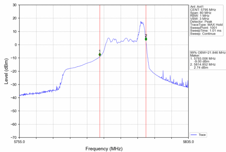
802.11ax(HEW40) HCH 5795MHz RU52 44 Ant1 NTNv
