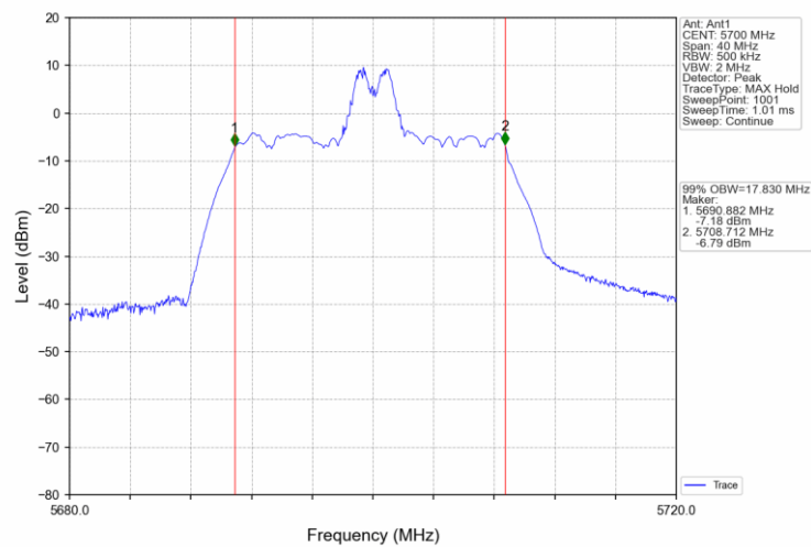
802.11ax(HEW20)_HCH_5700MHz_RU52_40_Ant1_NTNV
