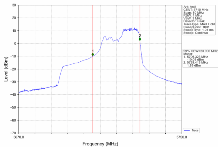
802.11ax(HEW40) HCH 5710MHz RU242_62 Ant1 NTNv
