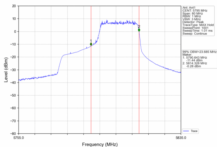
802.11ax(HEW40) HCH 5795MHz RU484_65_Ant1_NTNV
