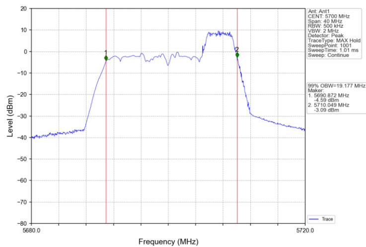
802.11ax(HEW20)_HCH_5700MHz_RU106_54_Ant1_NTNV
