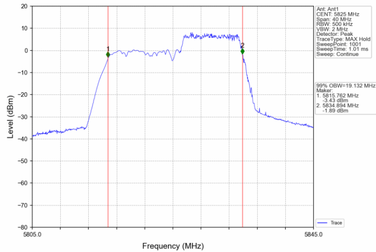
802.11ax(HEW20)_HCH_5825MHz_RU242_61_Ant1_NTNV
