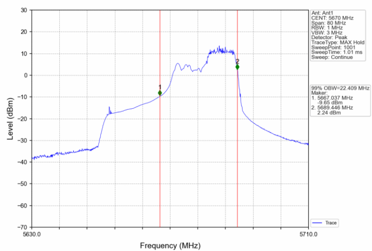
802.11ax(HEW40) HCH 5670MHz RU242 62 Ant1 NTNv
