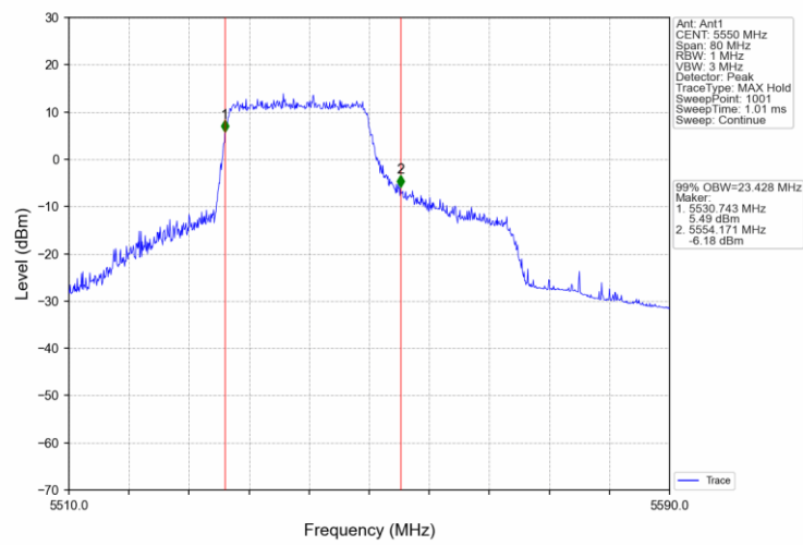
802.11ax(HEW40)_MCH_5550MHz_RU484_65_Ant1_NTNV
