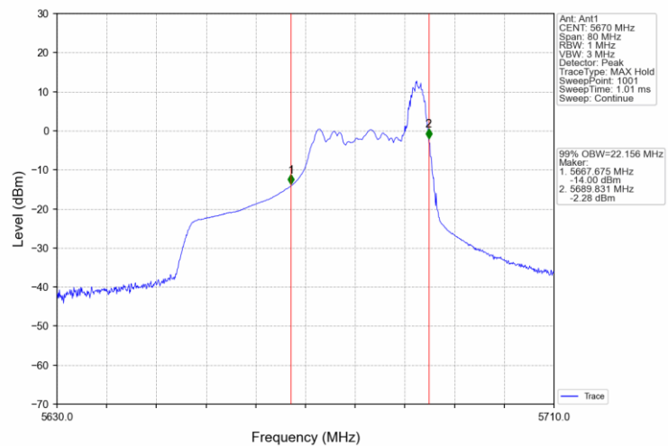
802.11ax(HEW40) HCH 5670MHz RU52 44 Ant1 NTNv
