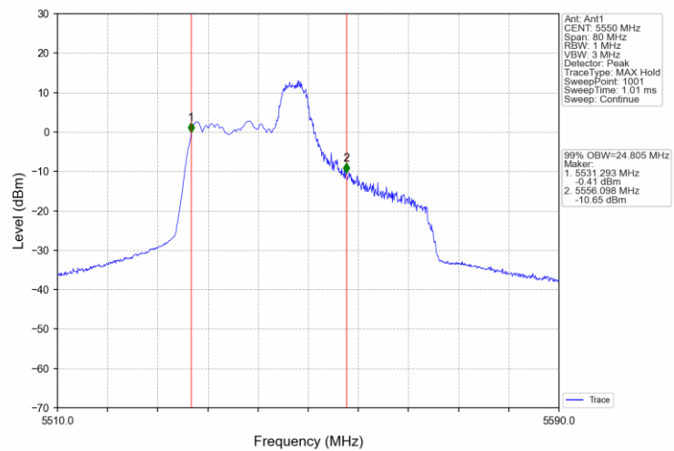
802.11ax(HEW40) MCH 5550MHz RU106 54 Ant1 NTNv
