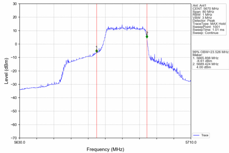
802.11ax(HEW40)_HCH_5670MHz_RU484_65_Ant1_NTNV
