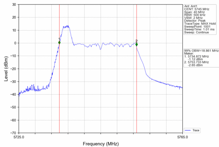
802.11ax(HEW20)_LCH_5745MHz_RU52_37_Ant1_NTNV
