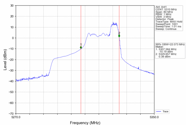
802.11ax(HEW40) HCH 5310MHz RU106_56 Ant1 NTNv
