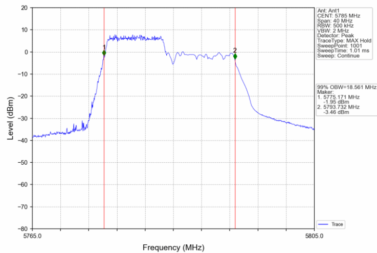
802.11ax(HEW20) MCH 5785MHz RU242_61 Ant1 NTNv
