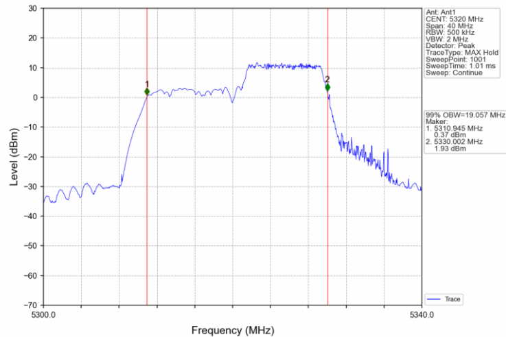
802.11ax(HEW20)_HCH_5320MHz_RU242_61_Ant1_NTNV
