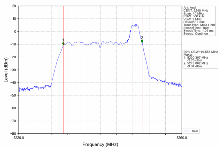
802.11ax(HEW20)_HCH_5240MHz_RU52_40_Ant1_NTNV
