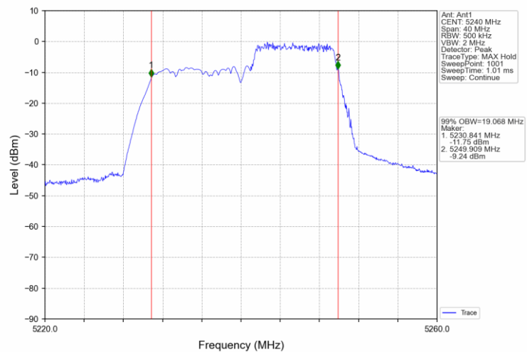
802.11ax(HEW20)_HCH_5240MHz_RU242_61_Ant1_NTNV
