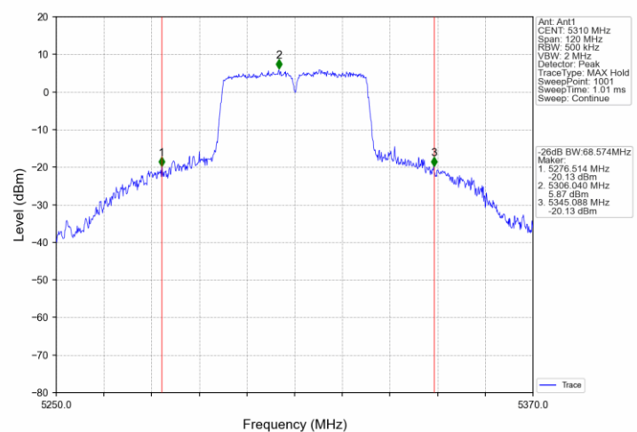
802.11ac(VHT40)_HCH_5310MHz_Ant1_NTNV
