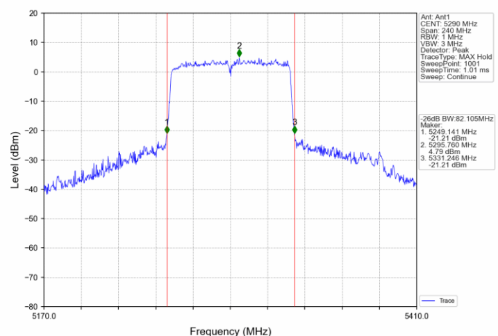
802.11ac(VHT80)_MCH_5290MHz_Ant1_NTNV
