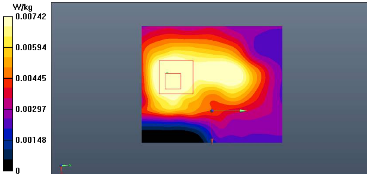
Fig.1 Bluetooth Head/Body
