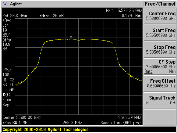
5580 MHz
