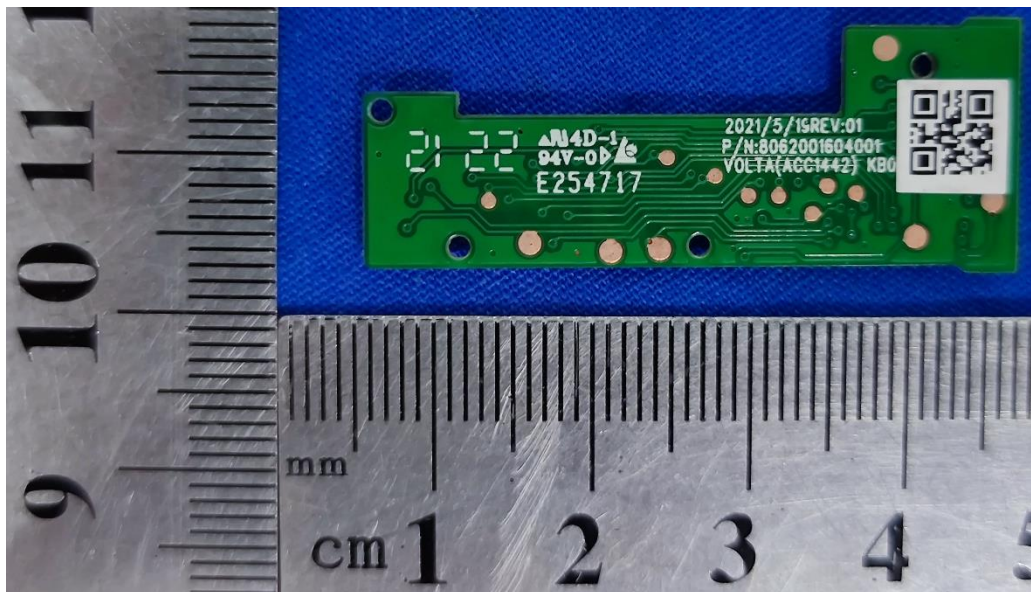
330-002-064 PCBA, KB board, Back, ACVT1
