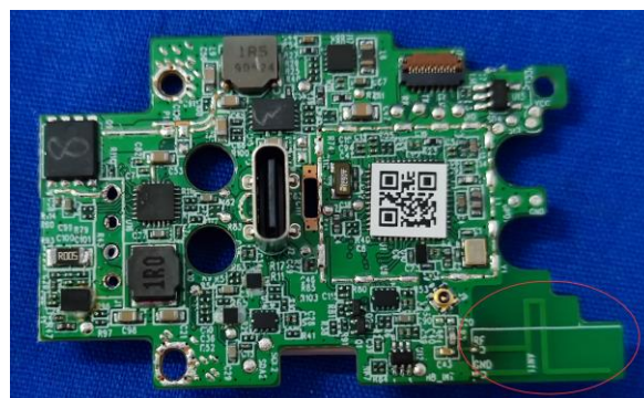
BT antenna location, ACVT1
