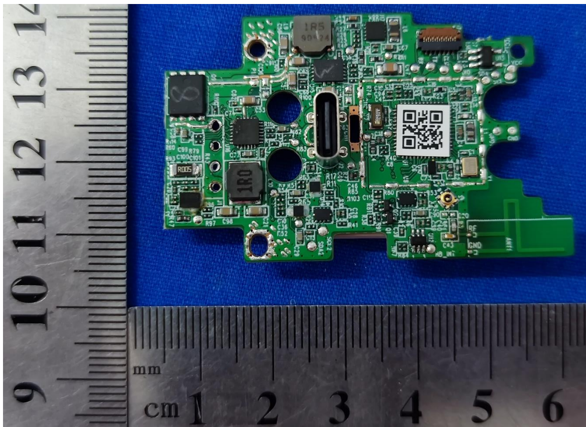
330-002-052 PCBA, MAIN board, Front, ACVT1
