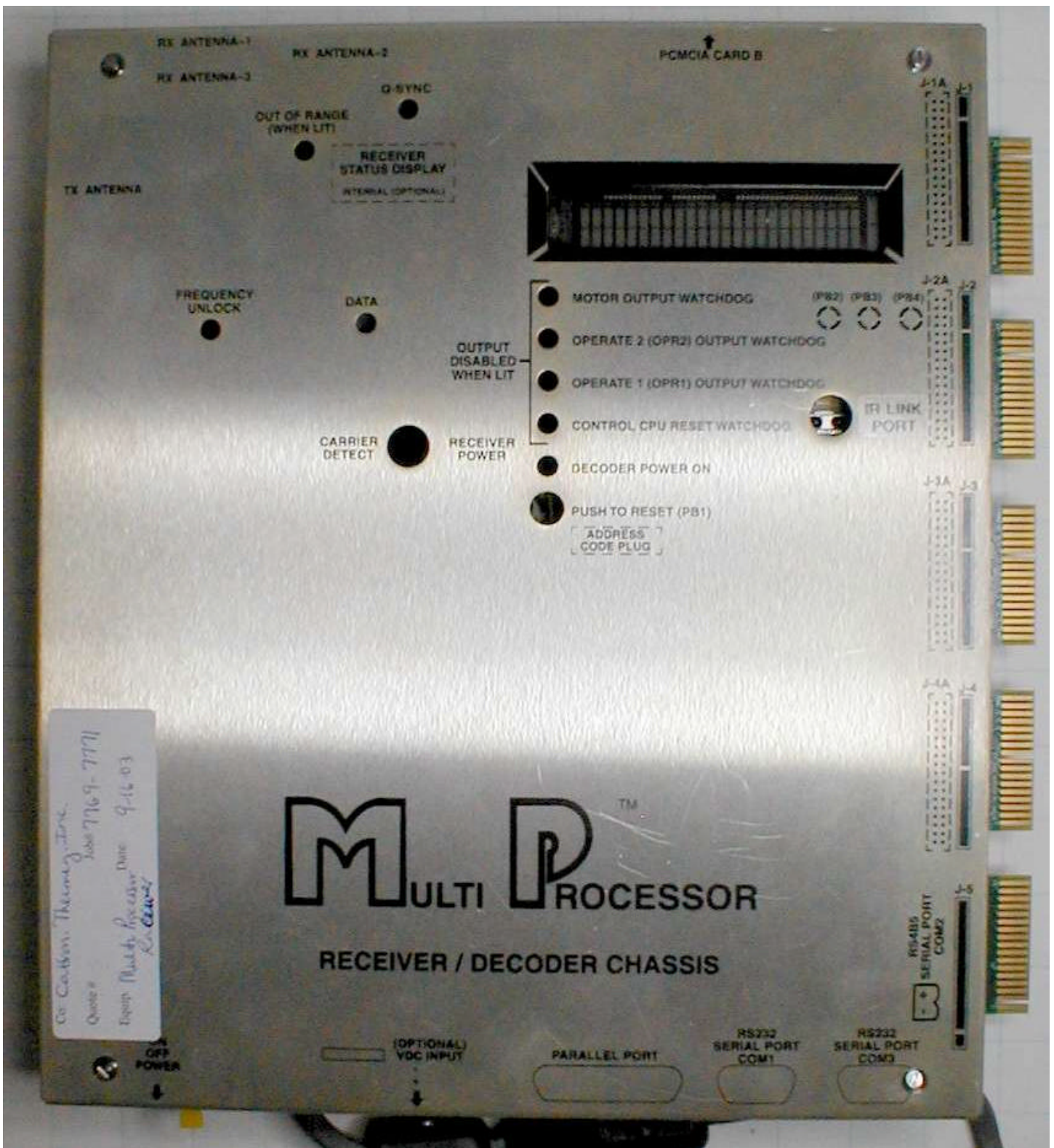
Front View
