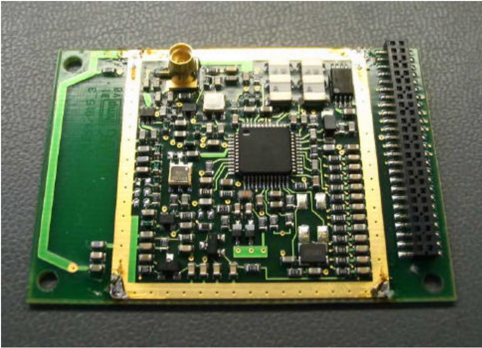
RF board – Shielding removed. Other side:
