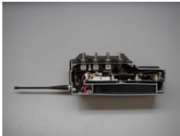
M840T-90HP OPEN (PCB shown)
