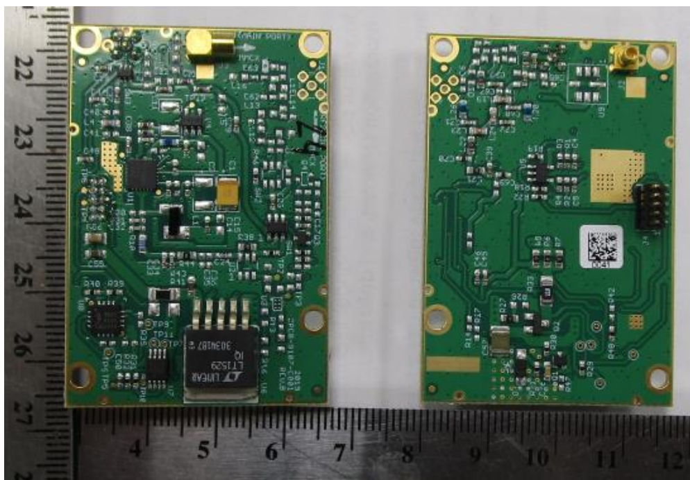
PA module TOP and BOTTOM view
