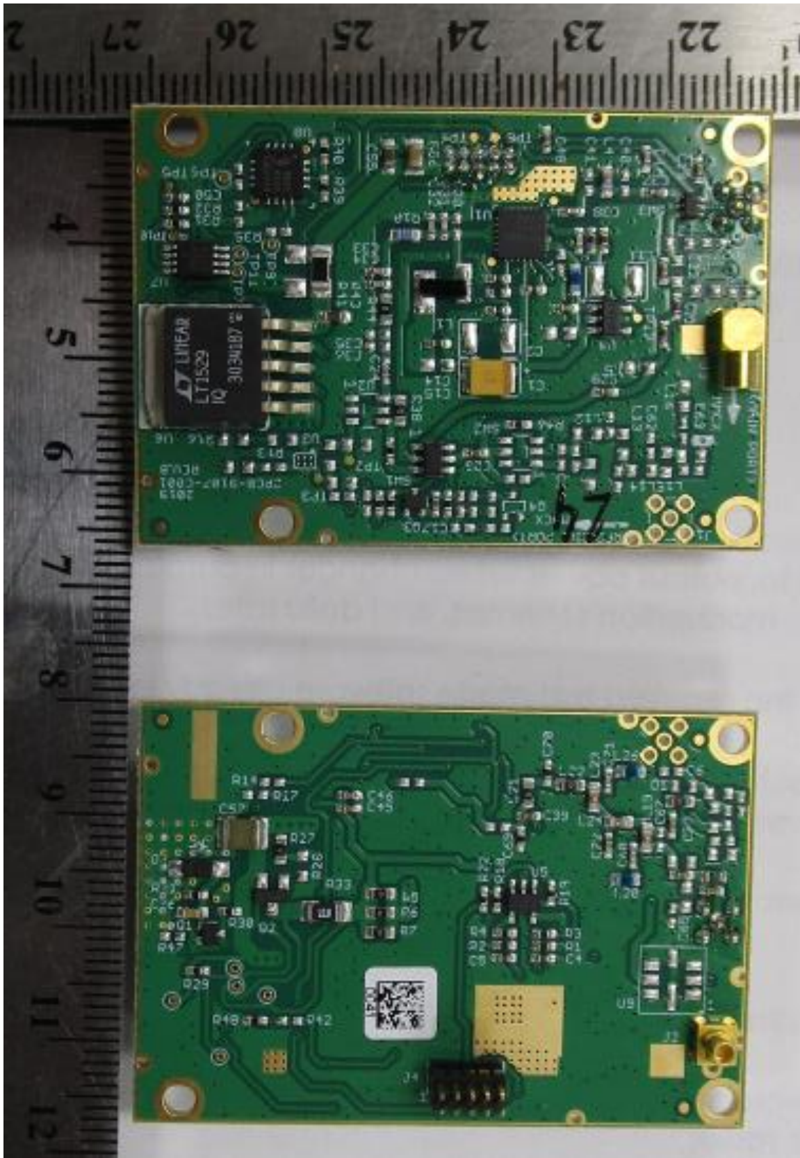
Power Amplifier module TOP and BOTTOM view
