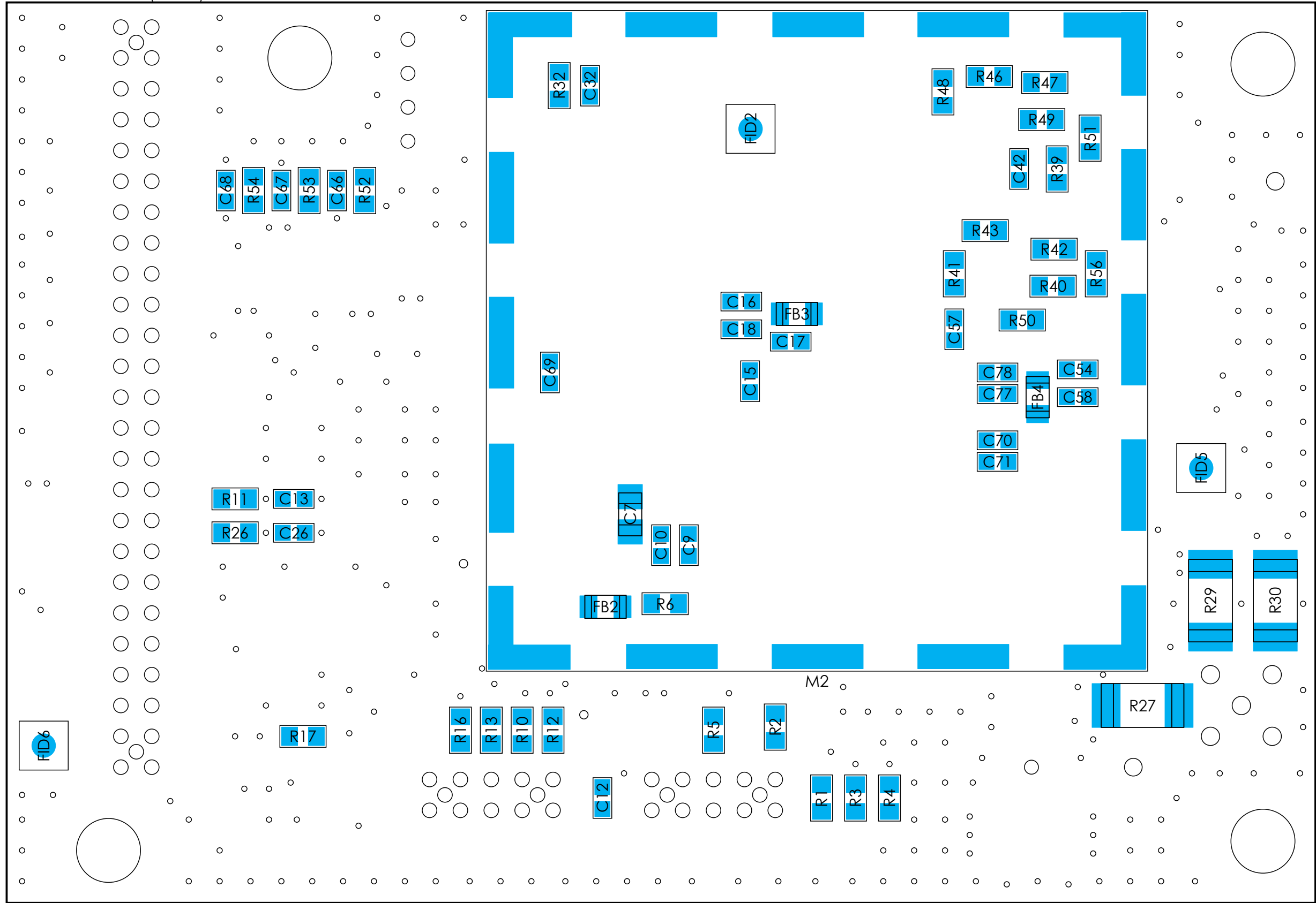
View from Bottom side (Scale 6)
