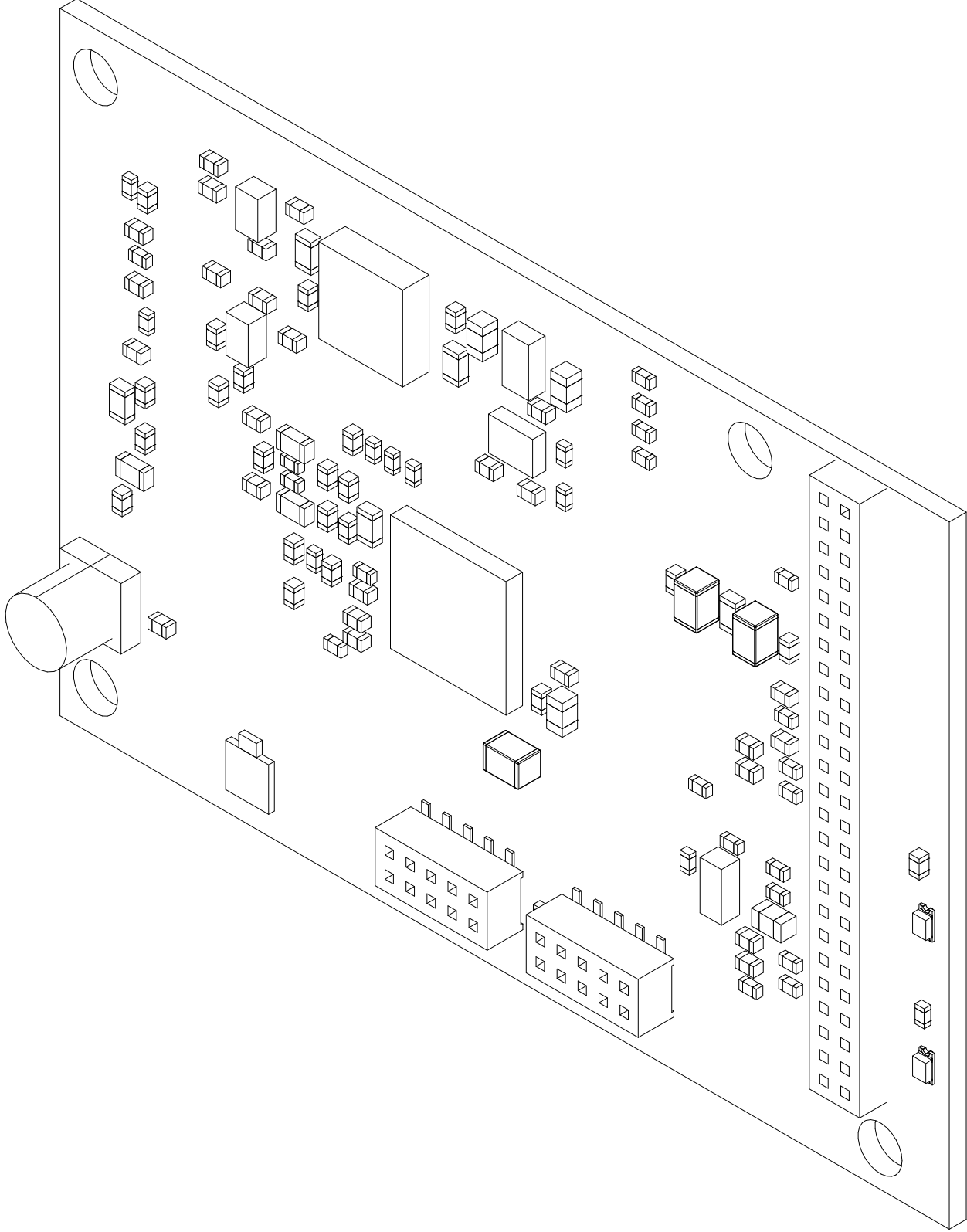
View from Top side (Scale 4:1)
