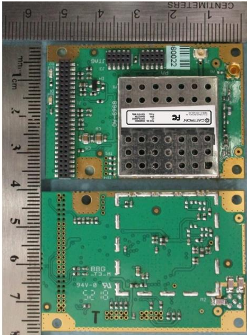
Transceiver module TOP and BOTTOM View with shielding And label location
