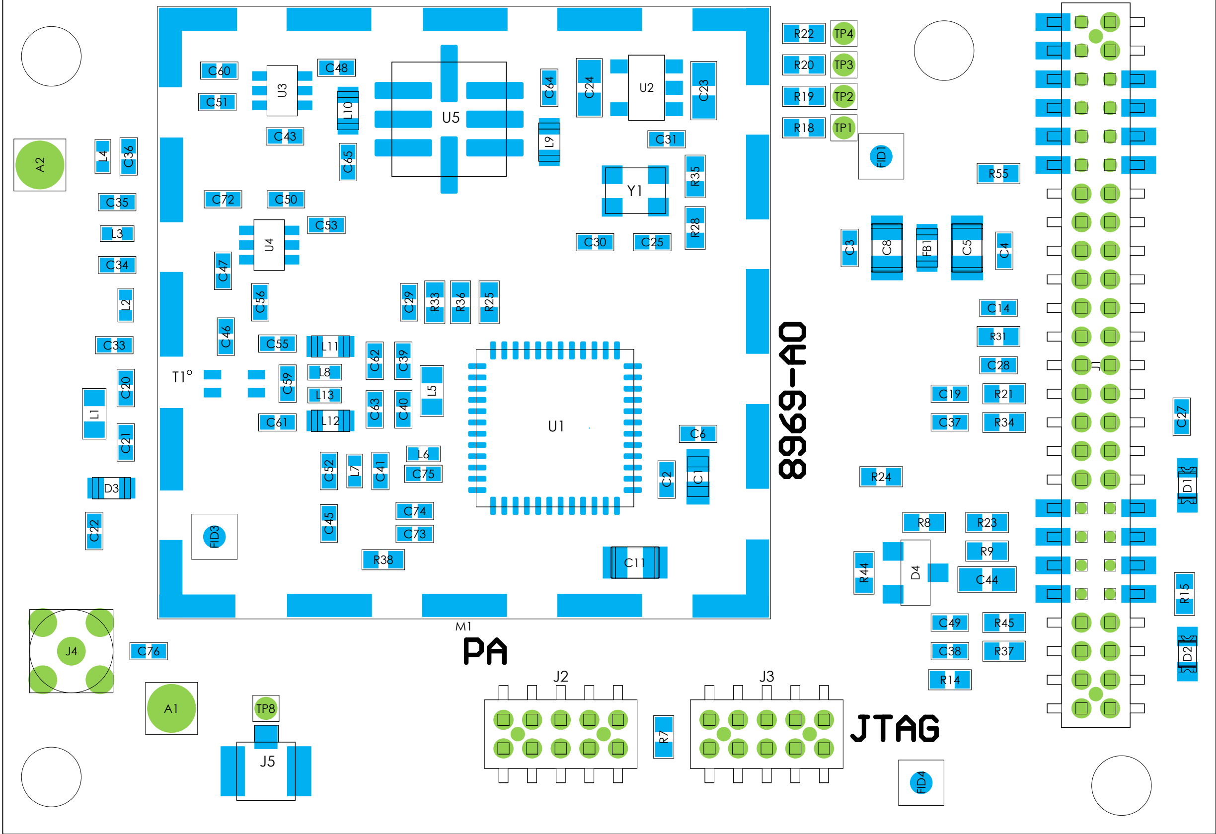
View from Top side (Scale 6)
