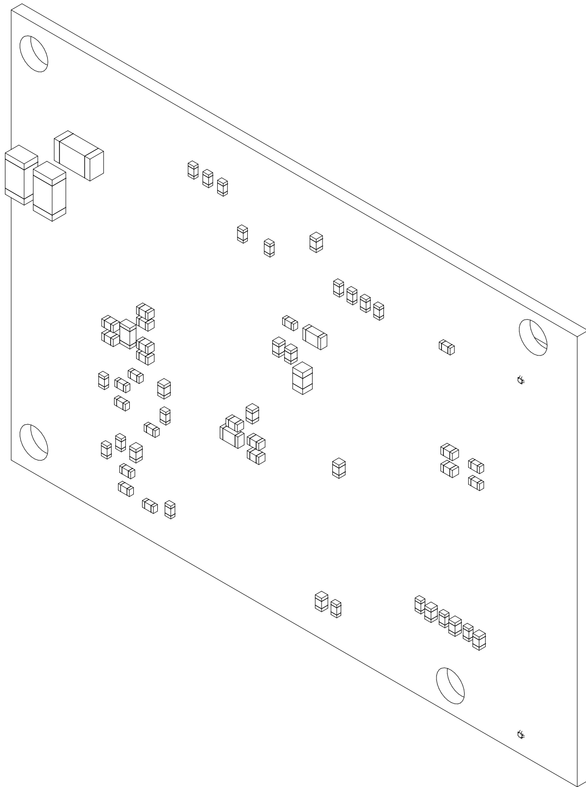
View from Bottom side (Scale 4:1)
