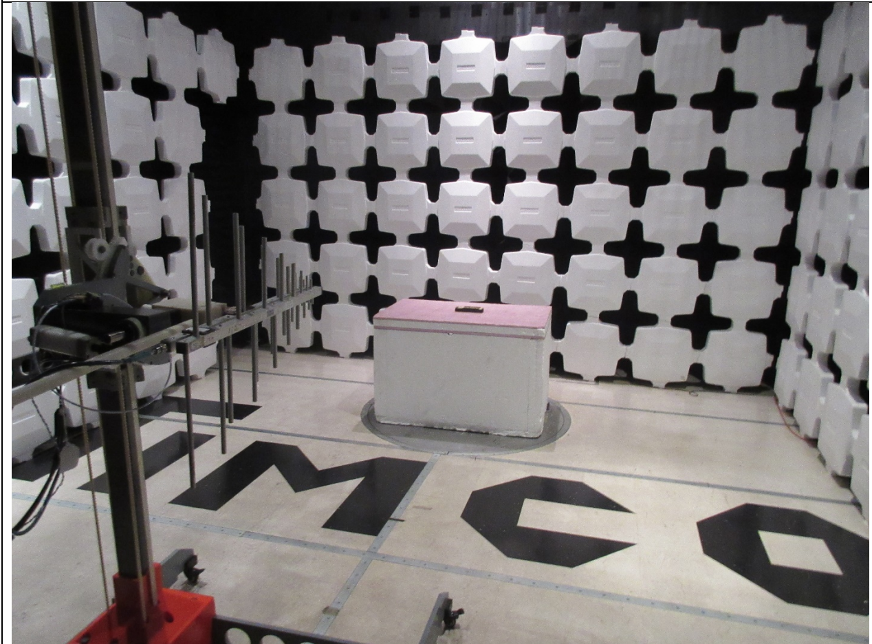
Occupied Bandwidth / Bandedge / Radiated Emissions Below 1 GHz Setup
