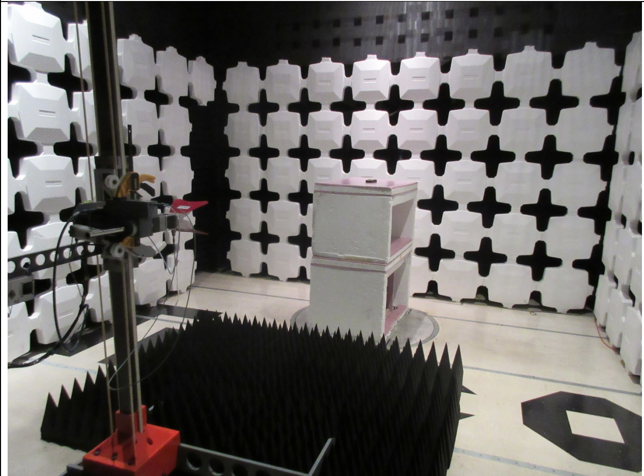
Radiated Emissions Above 1 GHz Setup
