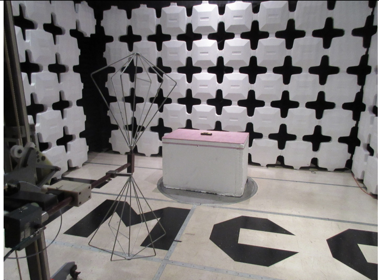
Radiated Emissions Final Setup
