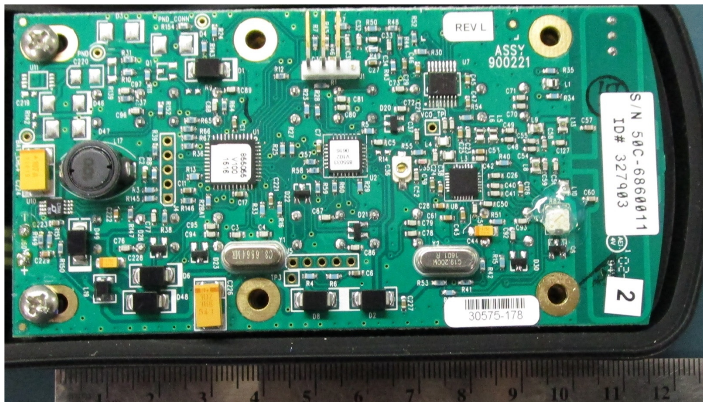
Bottom View
