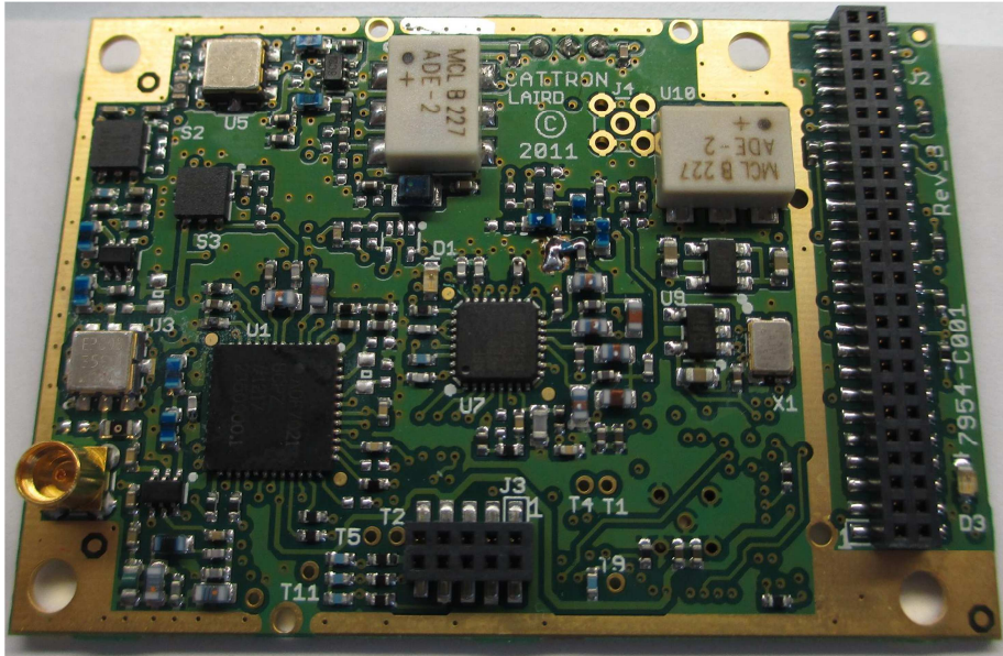
LRM 450MHz 79543TRX TOP without Shielding
