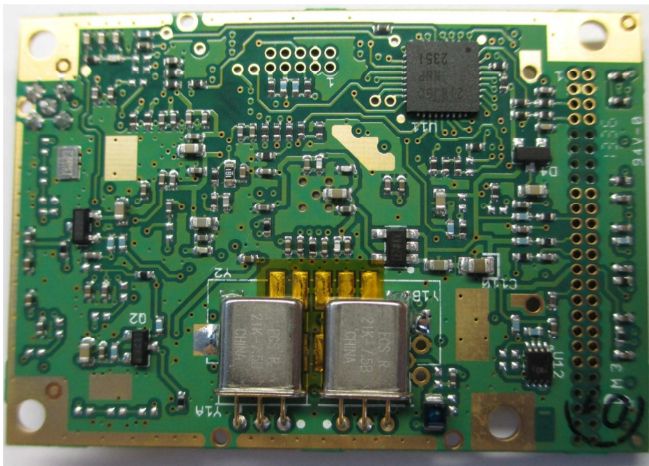
LRM 450MHz 79543TRX BOTTOM without Shielding
