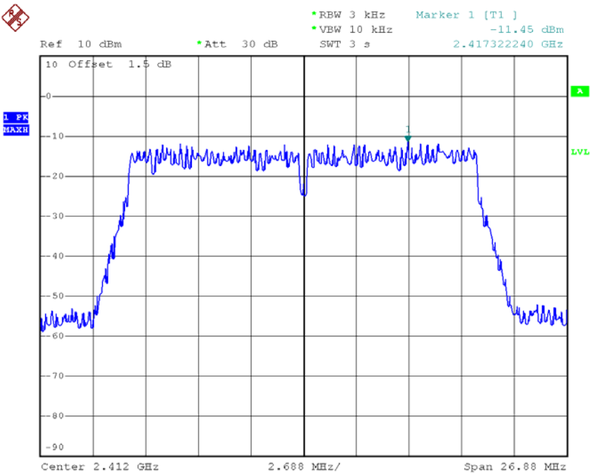
Mode 7 : PSD Plot on 802.11n Channel 01
