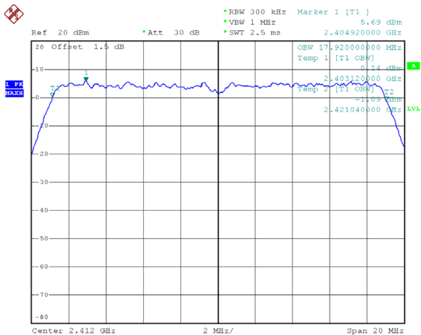
Mode 7 : 99% Occupied Bandwidth Plot on 802.11n Channel 01
