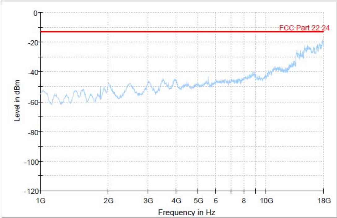
Field Strength of Spurious Radiated 1GHz-18GHz Horizontal
