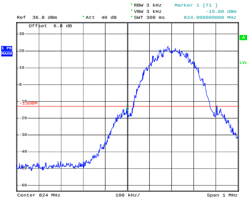
Lower Band Edge Plot on Channel 128
