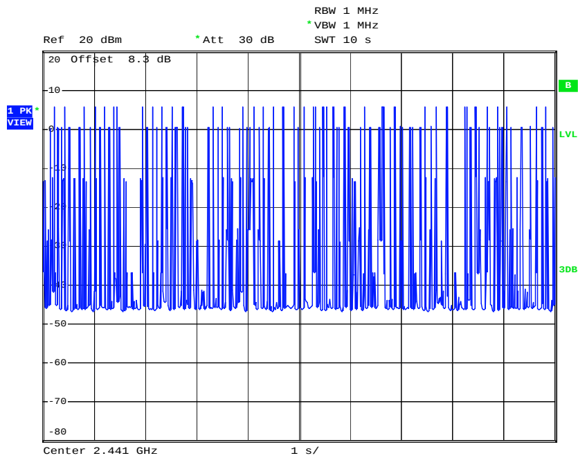
3DH3 Dwell Time (Count Pulses) Plot on Channel 39
