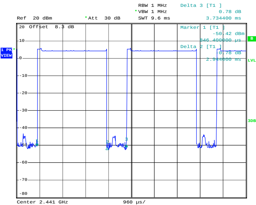
3DH5 Dwell Time (One Pulse) Plot on Channel 39
