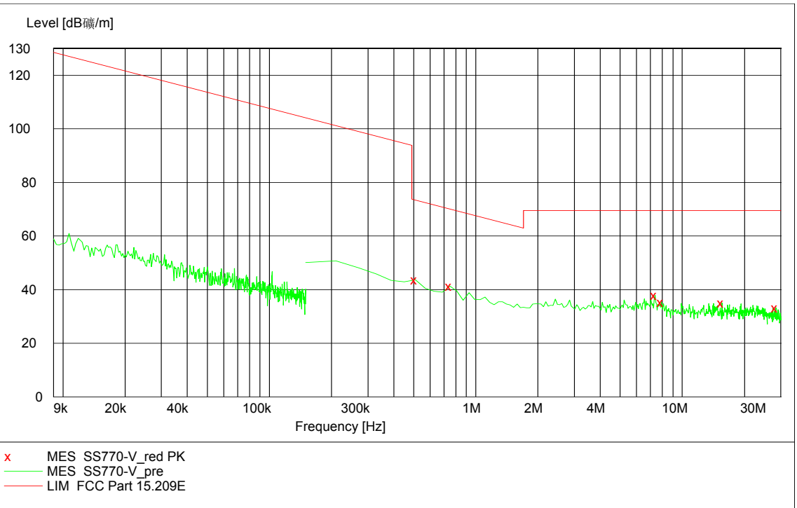
Radiated Emission Plot between 9 kHz ~ 30MHz (Vertical)
