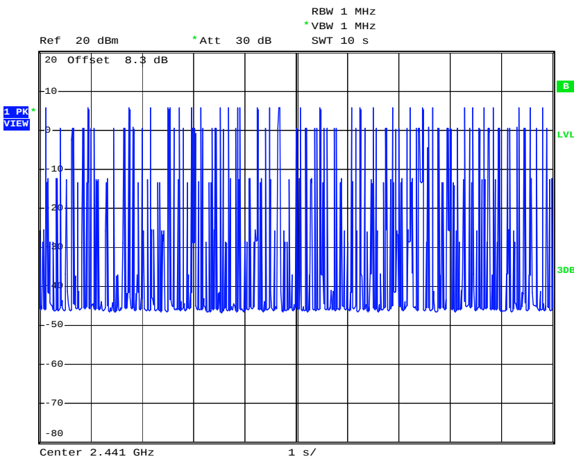
3DH5 Dwell Time (Count Pulses) Plot on Channel 39
