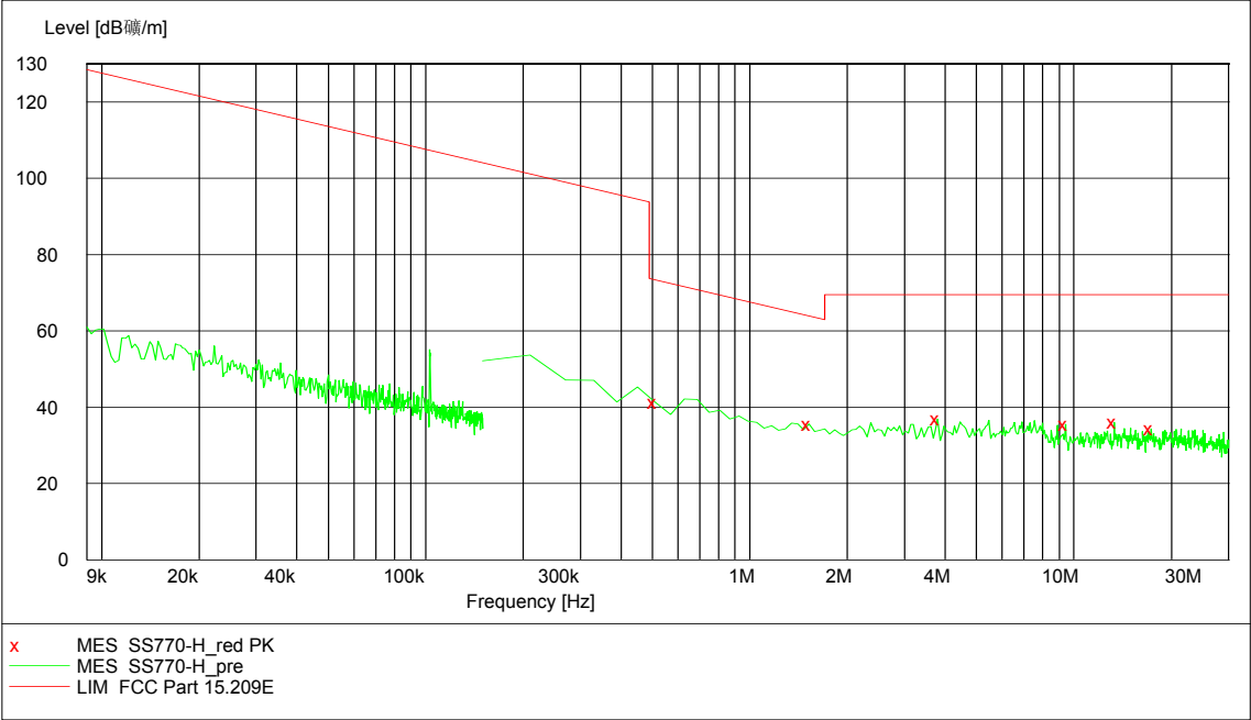
Radiated Emission Plot between 9 kHz ~ 30MHz (Horizontal)
