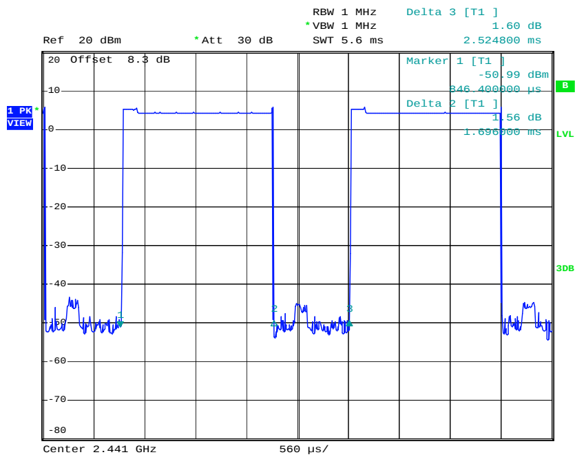
3DH3 Dwell Time (One Pulse) Plot on Channel 39
