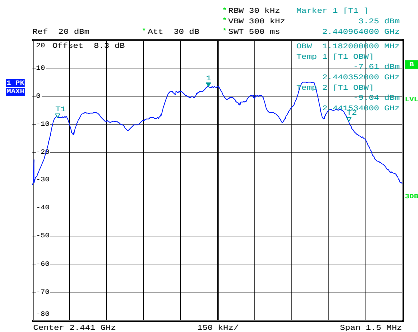
99% Occupied Bandwidth Plot on Channel 39
