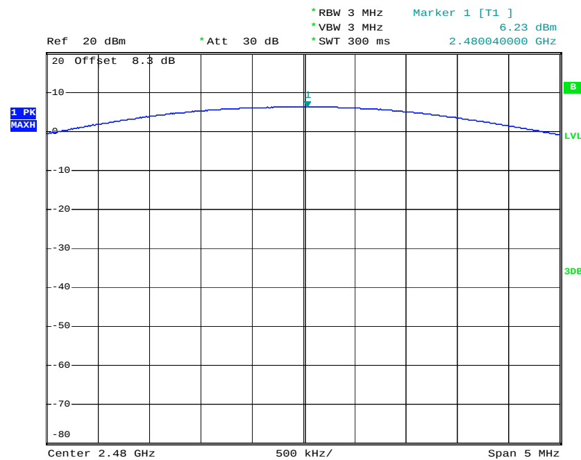
Peak Output Power Plot on Channel 78
