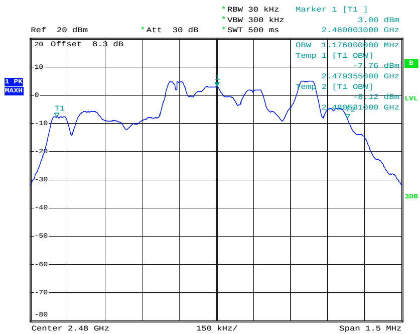
99% Occupied Bandwidth Plot on Channel 78
